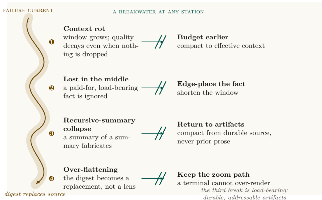
Figure 10: Context degradation is a current that becomes a cascade only when it passes every breakwater. Rot pressures compaction; naive compaction loses the middle; recursive summaries fabricate; and the operator-facing digest finally replaces its source. Any intervention stops the run, but the load-bearing one is station 3: compact from durable artifacts , so every new reading can be checked against an addressable claim, note, episode, or diff rather than a prior summary. Cost and truth fail together on this surface.
