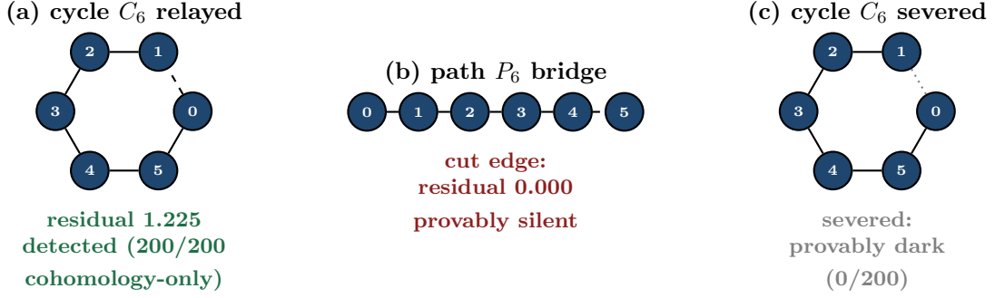
Figure 3: Regime diagram for the mechanism: (a) relayed cycle edge — residual 1.225, detected (200/200 cohomology-only); (b) cut edge — residual 0.000, provably silent; (c) severed cycle edge — provably dark (0/200). Detection requires the cycle and the relayed reports; each panel is one clause of the observability contract [internal, sheaf_harness_v2.py ].
