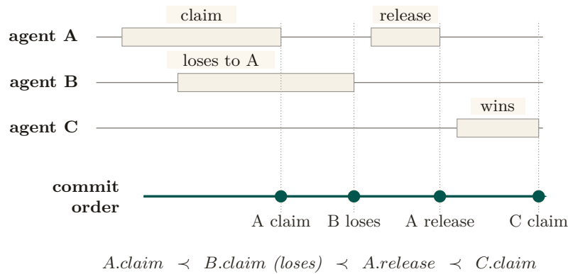
Figure 12: A real-time history and its extracted linearization. Operations overlap in caller time, but each receives one commit point on the single writer’s rail, and the linearization reads: A claims, B loses, A releases, C claims. The claim is conditional on one writer, no uncommitted reads, and replies after commit. [internal]
