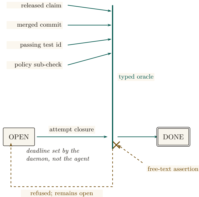
Figure 9: Typed evidence passes through a narrow closure aperture. A commitment closes as done only when the daemon can re-run a check from the finite oracle vocabulary: a released claim, merged commit, passing test id, or satisfied policy sub-check. A free-text assertion is refused and the commitment remains open. The deadline is set by the daemon, not the agent. [internal]
