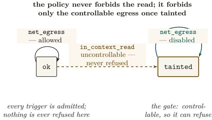
Figure 7: The compound policy’s supervisor as a two-state automaton, Schneider’s own Figure 1 for “no Send after a FileRead ” [4] with the states relabelled to this kernel’s alphabet. The uncontrollable trigger in_context_read is enabled — and never disabled — in both states, so the controllability criterion never has to refuse it; only the controllable effect event net_egress is disabled, and only after the taint transition fires. This is the constructive witness behind §8.3.1’s design rule: gate the channel, never the token. [internal]
