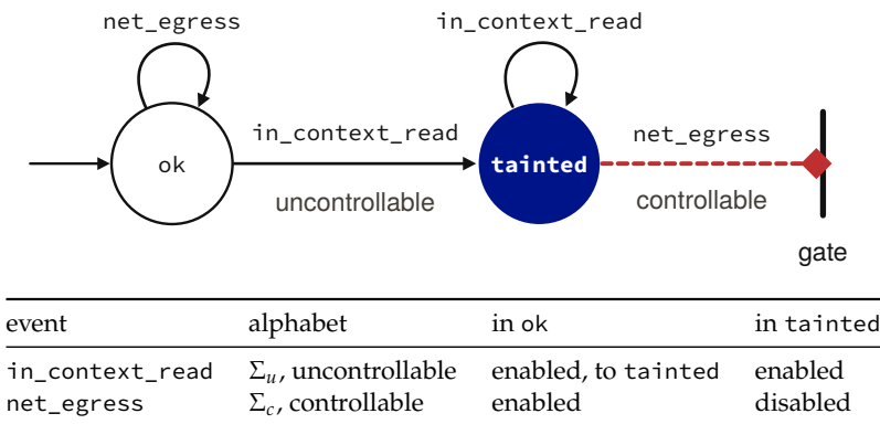
Figure 1.15: The taint automaton behind the sealed room: Schneider’s two-state security automaton for “no egress after an in-context read of a secret”, with his states relabelled. The read is uncontrollable, and the policy never tries to refuse it: it is enabled in both states and only records the taint. The one event the tainted state disables is net_egress , which the daemon mediates, so every uncontrollable event stays enabled and the policy is regimentable. Gate the channel, never the token [internal, b3_controllability.py].
