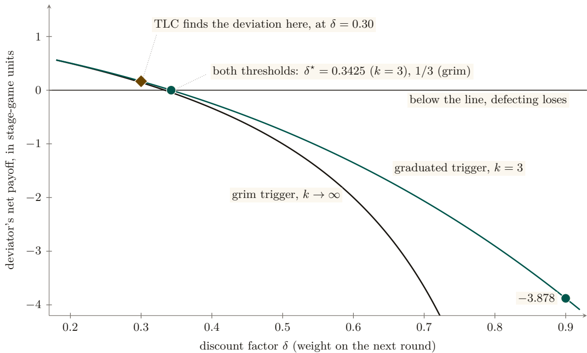
Figure 2: Net payoff to a player who defects once, against the discount factor, under the two punishment regimes of this section. The two curves cross zero 0.0092 apart — \delta^* = 0.3425 for the three-round graduated trigger, 1/3 for grim trigger — so bounding the punishment at three rounds costs almost nothing in the threshold. Away from the threshold the two regimes are not close at all: grim trigger’s punishment grows without bound and leaves the frame at \delta = 0.722 , where it reaches the axis floor, while the graduated trigger’s stays finite, reaching the chapter’s worked value of -3.878 at \delta = 0.9 . The marked point at \delta = 0.30 is the one discount factor whose model-checker transcript is committed — the session printed below — and its height, 0.166, is that run’s own closing margin, so the sign there, defecting still pays, is what the run reports. Both curves are the section’s own closed form at (c, d, p) = (3, 4, 1) , not a simulation [verified, proofs/economics/delta-threshold.z3 and claim_signaling_delta30.run.log ].
