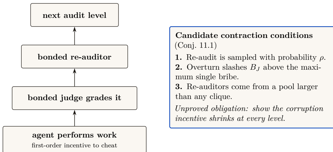
Figure 12: The rate-the-raters recursion. Conjecture 11.1 asks whether sampling, a slash exceeding the maximum bribe, and a conflict-free re-auditor pool larger than any clique make the incentive to corrupt each level strictly smaller than the level below. If proved, the tower would contract toward a finite honest fixed point. The paper names this as an unproved obligation rather than depicting the desired result as established.
