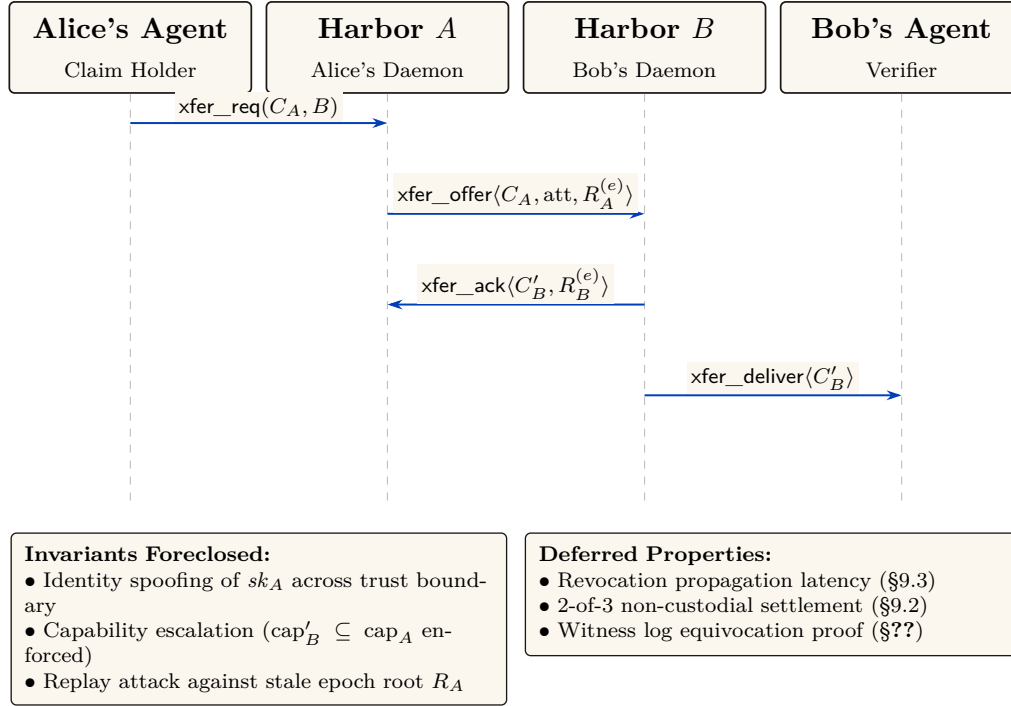
Figure 6: The four-message cross-harbor capability transfer ceremony. The critical property is that no message after (3) needs to reach back to Harbor A in the hot path: C'_B is verifiable under sk_B alone, which is why federation does not turn every authorization into a synchronous inter-machine round trip. The epoch root R_A^{(e)} bound into the envelope is the load-bearing primitive — a revocation issued by A after epoch e invalidates C'_B as soon as the new R_A^{(e+1)} reaches the witness log that B audits.
