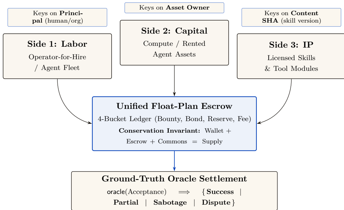
Figure 2: The three-sided market. Labor, capital (rented agents), and IP (licensed skills) are three distinct incentive constraints — not three UI tabs — that all settle on a single float-plan escrow, so conservation holds globally without a second ledger. This is the categorical heart of the design: the three sides are isomorphic at the conservation object (the escrow) and non-isomorphic at the identity object (each side keys reputation on a different entity, the dashed band). Calling it “one structure, three decorations” without that qualifier is a decorative-analogy failure. The rider is mandatory: the market is three-sided by design and two-sided in shipped reality, because sides 2 and 3 presuppose a non-forgeable, durable identity (§6). The economics per side: labor’s margin is bounty — slashed sub-bonds — fee; capital’s renter holds the runtime jail while the owner bears reputation; IP is metered with clawback, paid only on green settlement. The escrow and its conservation invariant are implemented and property-tested.
