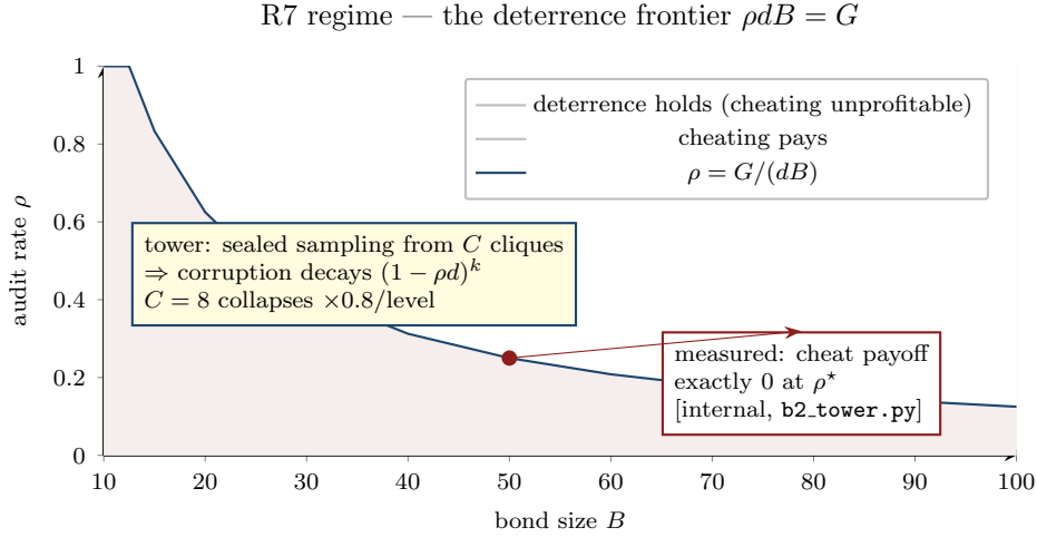
Figure 2: The regime diagram: the deterrence frontier \rho dB = G in the (\text{bond } B, \text{audit rate } \rho) plane at G=10 , d=0.8 . Above the curve \rho = G/(dB) , cheating is unprofitable; below it, cheating pays. The marked point is the running example (B, \rho^*) = (50, 0.25) , where the measured cheat payoff is exactly zero [internal, b2_tower.py ]. The inset records the tower consequence of §5: sealed sampling from C cliques drives surviving corrupt value down as (1 - \rho d)^k , a \times 0.8 -per-level collapse at C=8 .
