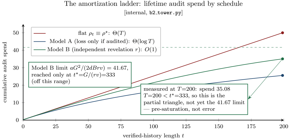
Figure 3: Cumulative audit spend against verified-history length t under the three incentive-compatible schedules of Theorem 3, at the running parameters. Flat auditing (shipred) grows linearly; Model A (harborblue) grows logarithmically; Model B (seagreen) approaches the closed-form limit aG^2/(2dBrv) = 41.67 but has not reached it by the measured horizon T=200 , since saturation requires t^* = G/(rv) = 333 — the gap between the measured 35.08 and the limit is pre-asymptotic, not error [internal, b2_tower.py].
