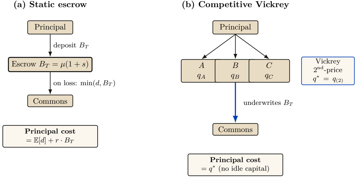
Figure 4: Static escrow vs. competitive Vickrey auction. Both regimes underwrite the same coverage B_T = \mu(1 + s) ; only the financing mechanism differs. In (a) the principal ties up B_T for the coverage period, paying an opportunity cost r \cdot B_T . In (b) insurers compete; the principal pays only the second-lowest bid q^* . The competitive regime Pareto-dominates the static one under the welfare assumptions of §7.5.8 below.
