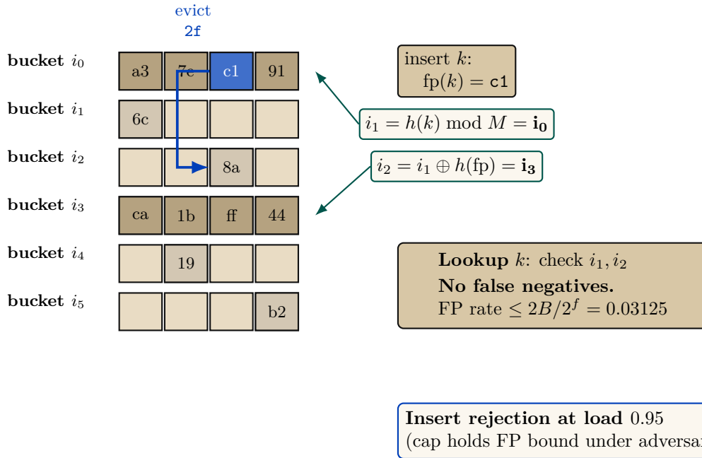
Figure 5: Cuckoo-filter revocation gate (Fan et al. [25]) with the load-factor ceiling that defeats the pollution attack. Insert lands at either of two candidate buckets i_1, i_2 = i_1 \oplus h(fp) ; on full, evict and re-insert at the kicked fingerprint’s alternate. Insert rejection at 0.95 caps occupancy inside the regime where the false-positive bound holds.
