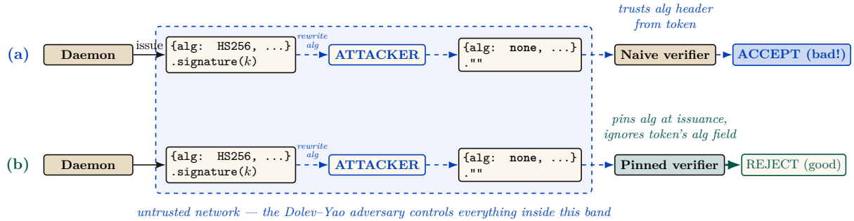
Figure 3: Algorithm-confusion attack and the pinned-verifier defense. The dashed band is the chapter’s trust boundary: the daemon and the verifier sit outside it, and everything inside it is under the control of the Dolev–Yao adversary of §5.1, who may read, rewrite, or inject any token in flight. (a) A naive verifier trusts the alg field of the incoming token; an attacker inside the band rewrites alg=HS256 to alg=none , strips the signature, and the verifier accepts an unauthenticated message. (b) The pinned verifier records the issuance algorithm out-of-band — across the boundary, where the adversary cannot reach — then re-checks each token against the pinned algorithm rather than the token’s self-described one. The ProVerif model encodes both verifiers and shows the naive path produces a counter-trace witness for the rewrite, while the pinned path admits no such trace. Runtime conformance: 5 attack patterns + 2 controls, all pass.
