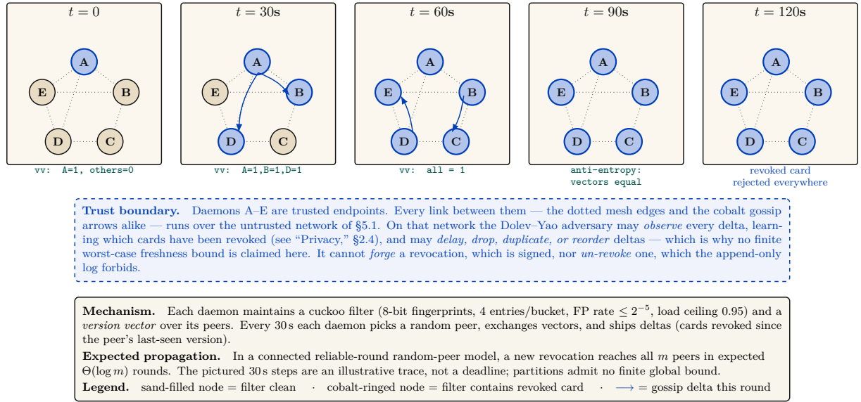
Figure 6: Gossip-synchronized revocation across a five-daemon mesh. At t = 0 daemon A locally revokes a Harbor Card (its filter and revocation table). Anti-entropy gossip ships deltas to random peers every 30 s. Expected \Theta(\log m) propagation requires the stated connected reliable-round model; the panels show one possible execution, not a worst-case time guarantee. Version vectors make duplicate and reordered deltas idempotent once delivered, but do not heal an unbounded partition. The dashed strip beneath the panels states the trust boundary the panels themselves cannot draw: the daemons are trusted, every wire between them is not.
