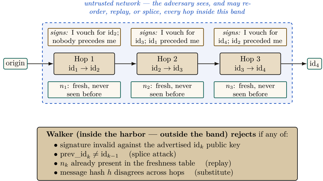
Figure 4: Multi-hop delegation walker. Each hop k signs the binding tuple (n_k, id_{k-1}, id_{k+1}, h) under Ed25519 — written sign_{id_k}(\text{hopBind}(n_k, id_{k-1}, id_{k+1}, h)) in Algorithm 3 — where h is the message hash that must remain constant across the chain; the boxes above each hop say in words what that tuple asserts. The dashed band is the trust boundary of §5.1: the whole chain is adversary-visible in transit, which is precisely why each hop must bind its neighbours rather than merely follow them. The walker runs inside the harbor, verifies depth- N chains against a nonce-freshness table, and rejects splices, replays, hop-swaps, and substitution. Runtime: lib/delegation-chain.ts ; ProVerif conformance test passes 17 / 17.
