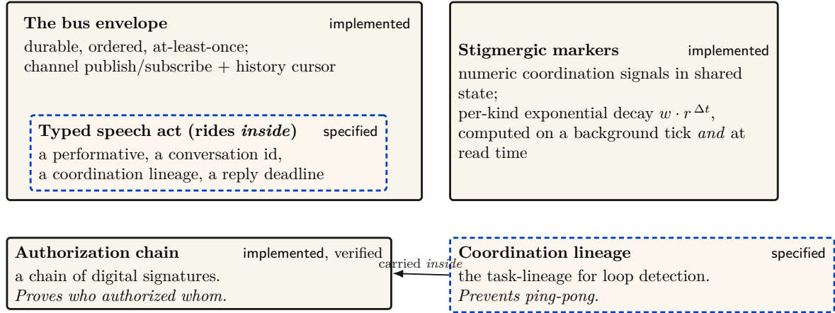
Figure II.6: The communication organ. The bus envelope — durable, ordered, at-least-once, history-cursored ( implemented ) — is the carrier into which the typed speech act is layered; the kernel ships the envelope, the coordination layer ships the semantics that ride inside it. Stigmergic markers implement coordination with per-kind exponential decay computed both on a background tick and at read time , so the anti-blackboard-rot property is provided by the substrate rather than left to discipline. Finally, the figure fixes a dangerous naming collision — never write bare “delegation chain,” it is two objects: the authorization chain is the hop-bound, attenuation-monotonic, anti-replay chain of signatures that proves who authorized whom ; the coordination lineage is the coordination object that prevents ping-pong — a different thing entirely, carried inside the authorization chain.
