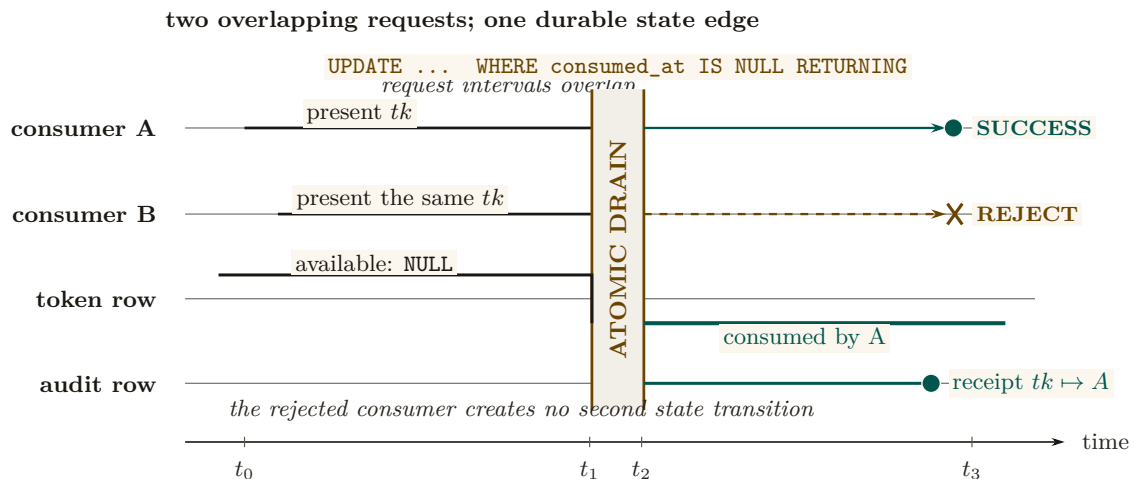
Figure 9: Single-use redemption is a concurrency property, not a two-arrow icon. Two consumers present the same account-bound token during one overlap window. Both requests reach the same serialized SQL update, but the token row has only one falling edge: the first transaction changes consumed_at from NULL and returns a row; the second observes the durable state and returns none. The audit rail records the winning consumer without creating another success path.
