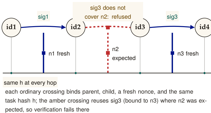
Figure 2.4: The delegation chain as a signed provenance braid across four identities id1–id4. Ordinary hops 1 and 3 bind parent, child, a fresh nonce (n1, n3), and the shared task hash h below. Hop 2 shows a splice attack: an attacker moves the legitimate signature sig3 (computed over id3, id4, and n3) into the id2–id3 position, where the verifier expects a signature over n2; the check fails at exactly that crossing, so the discontinuity is visible at one adjacent-identity boundary rather than anywhere else in the chain. [internal]
