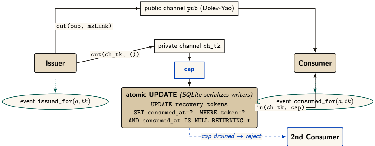
Figure 9: Magic-link single-use atomicity. The SQL UPDATE ...WHERE consumed_at IS NULL RETURNING is the runtime analogue of the ProVerif private-channel cap : SQLite serializes concurrent writers, so the first caller drains the cap and the second consumer’s transaction returns zero rows. Verified properties: injective single-use ( \text{inj-event}(\text{consumed\_for}) \Rightarrow \text{inj-event}(\text{issued\_for}) ) and binding.
