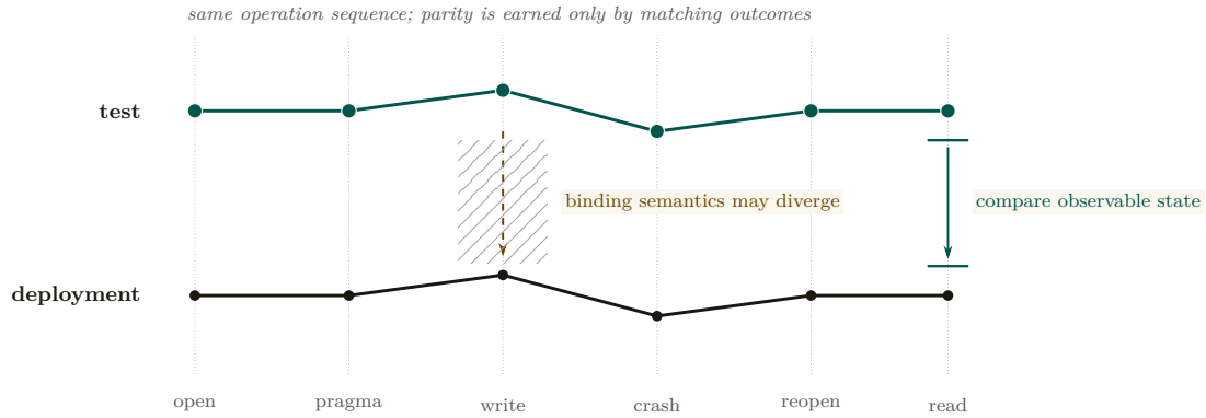
Figure 1.14: Runtime parity as a trajectory comparison. The same operation sequence is applied to the test binding and to the compiled deployment daemon; the harness must compare observable state after reopen, not merely confirm that both programs build. The hatched gap is the unproved surface where pragma, locking, or checkpoint semantics can diverge. A shim aligns interfaces, but only booting the deployment runtime and differential testing can collapse that gap into a verified invariant.
