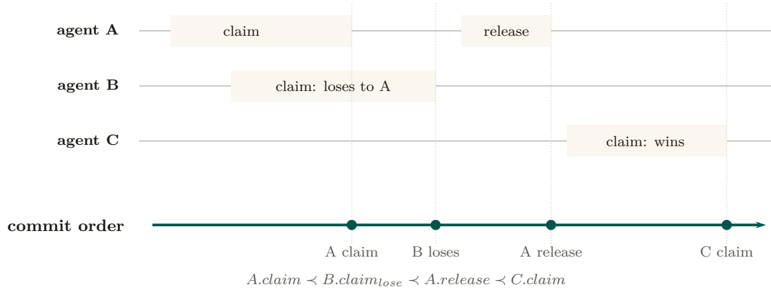
Figure 1.13: A real-time history and its extracted linearization. Operations may overlap in caller time, but each receives one commit point on the single writer’s rail. Those points explain the observable result without a prose table: A wins, B overlaps but loses to the recorded holder, A releases, and only then can C win. The claim is conditional on one writer, no uncommitted reads, and replies after commit; a bypass would destroy the correspondence.
