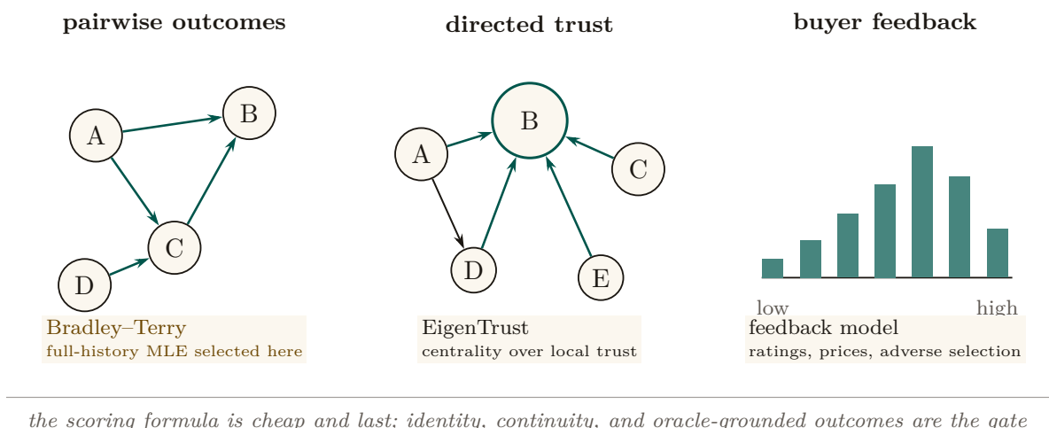
Figure 4.8: Estimator families are keyed to signal topology. Pairwise wins form a comparison graph and call for Bradley-Terry; a complete harbor history supports the full-history fit rather than streaming Elo. Directed local trust forms a network and calls for EigenTrust. Buyer ratings and price effects form a feedback distribution and call for marketplace models. These are not interchangeable score recipes. None repairs a forgeable identity or an agent-authored oracle: the trustworthy substrate still comes first.
