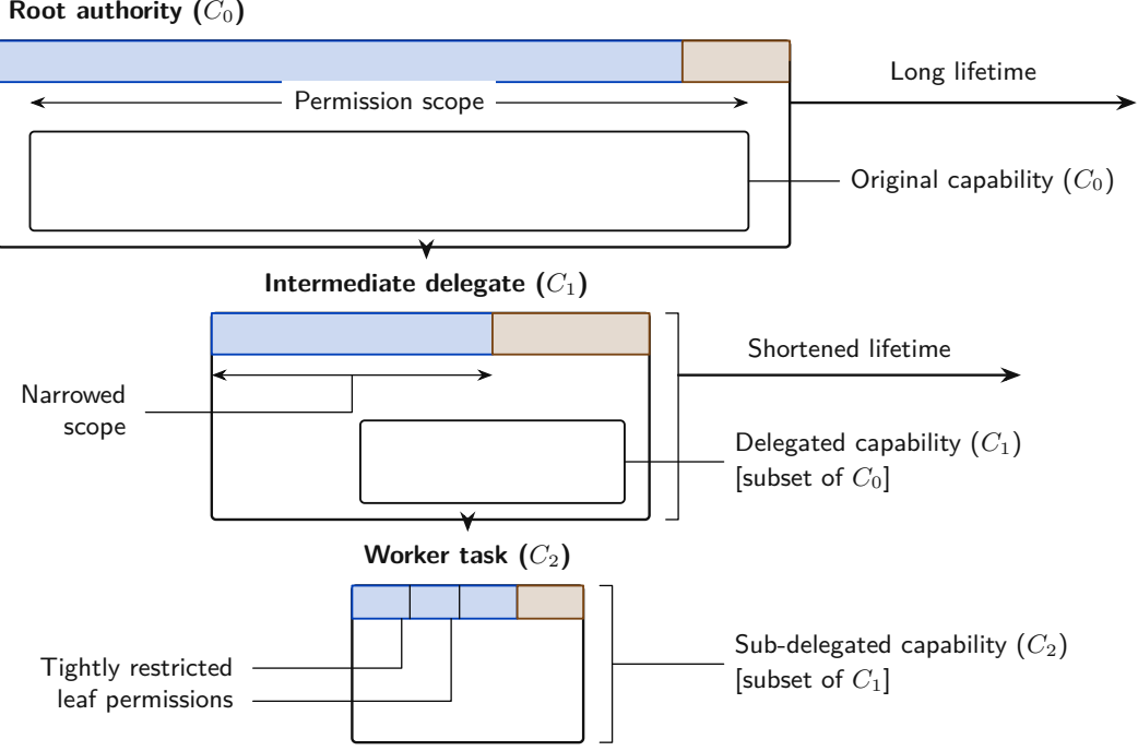
Figure 2: Proposition 2 Mechanics: Monotonic Capability Attenuation. Chained cryptographic capability tokens enforce monotonic restriction at every delegation hop. An intermediate delegate can append attenuating caveats (narrowing path scopes, reducing budgets, and shortening TTLs), but can never widen authority or extend parent lifetimes ( C_0 \supset C_1 \supset C_2 ).
