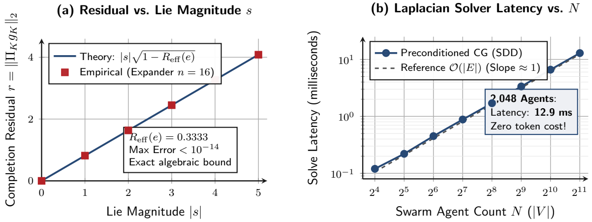
Figure 7: Numerical verification of Theorems CR-1 through CR-3 on synthetic expander meshes conforming to Swiss Modern Systems Graphics. (a) Observed residual r against lie magnitude s on a 16-agent mesh ( R_{\text{eff}} = 1/3 ), confirming the closed form r = |s|\sqrt{1 - R_{\text{eff}}(e)} with relative error < 10^{-14} . (b) Empirical solve latency of SDD Laplacian preconditioned CG solver from N = 16 to N = 2,048 agents, confirming near-linear scaling ( \sim 12.9 ms at 2,048 nodes).
