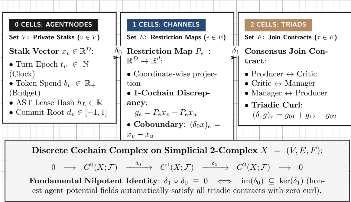
Figure 3: The Rosetta Stone conforming to Swiss Modern Systems Graphics: exact algebraic translation from multi-agent swarm primitives into cellular sheaves and simplicial complexes over cell complex X = (V, E, F) .
