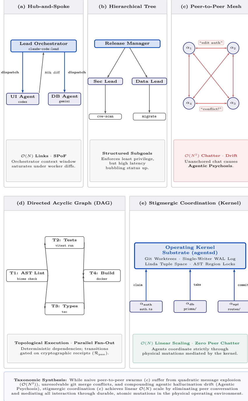
Figure 10: Taxonomy of Multi-Agent Swarm Topologies. While naive peer-to-peer swarms suffer from \mathcal{O}(N^2) message explosion, git merge conflicts, and agentic hallucination drift, the Stigmergic Blackboard coordinates agents via environmental state mutations mediated by the authoritative operating kernel.
