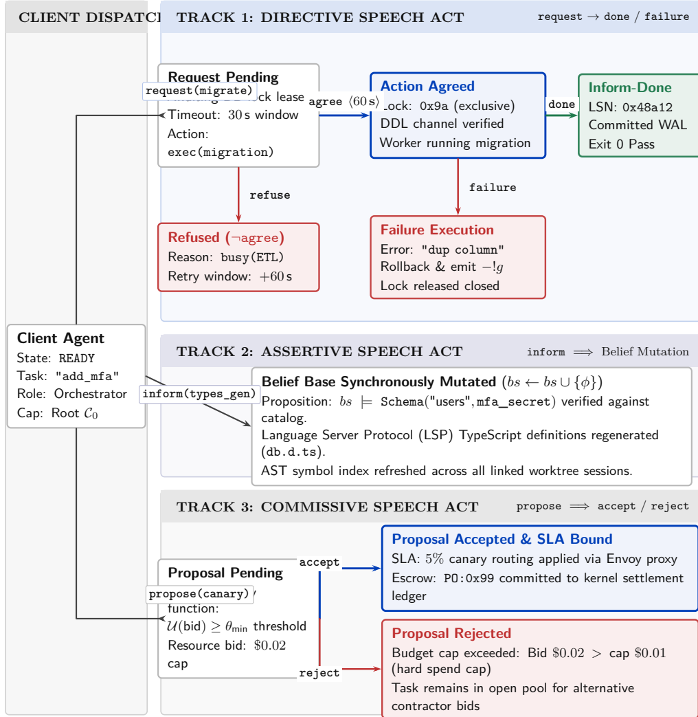
Figure 4: FIPA-00037 Communicative Speech Act state transition machine, populated with practical software engineering payloads. Top: Directive request lifecycle executing an atomic database migration under lock arbitration. Middle: Assertive inform directly mutating an agent’s belief base. Bottom: Commissive propose negotiating an SLA for canary deployment routing.
