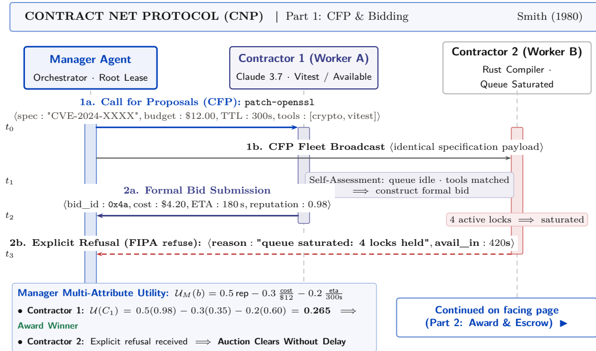
Figure 5: Smith’s (1980) Contract Net Protocol (Part 1 of 2: Task Announcement & Bidding; continued on facing page 21). An Orchestrator broadcasts a Call for Proposals (CFP) to patch a critical dependency CVE across competing agent workers. Competing workers assess tools and queue capacity to submit bids.
