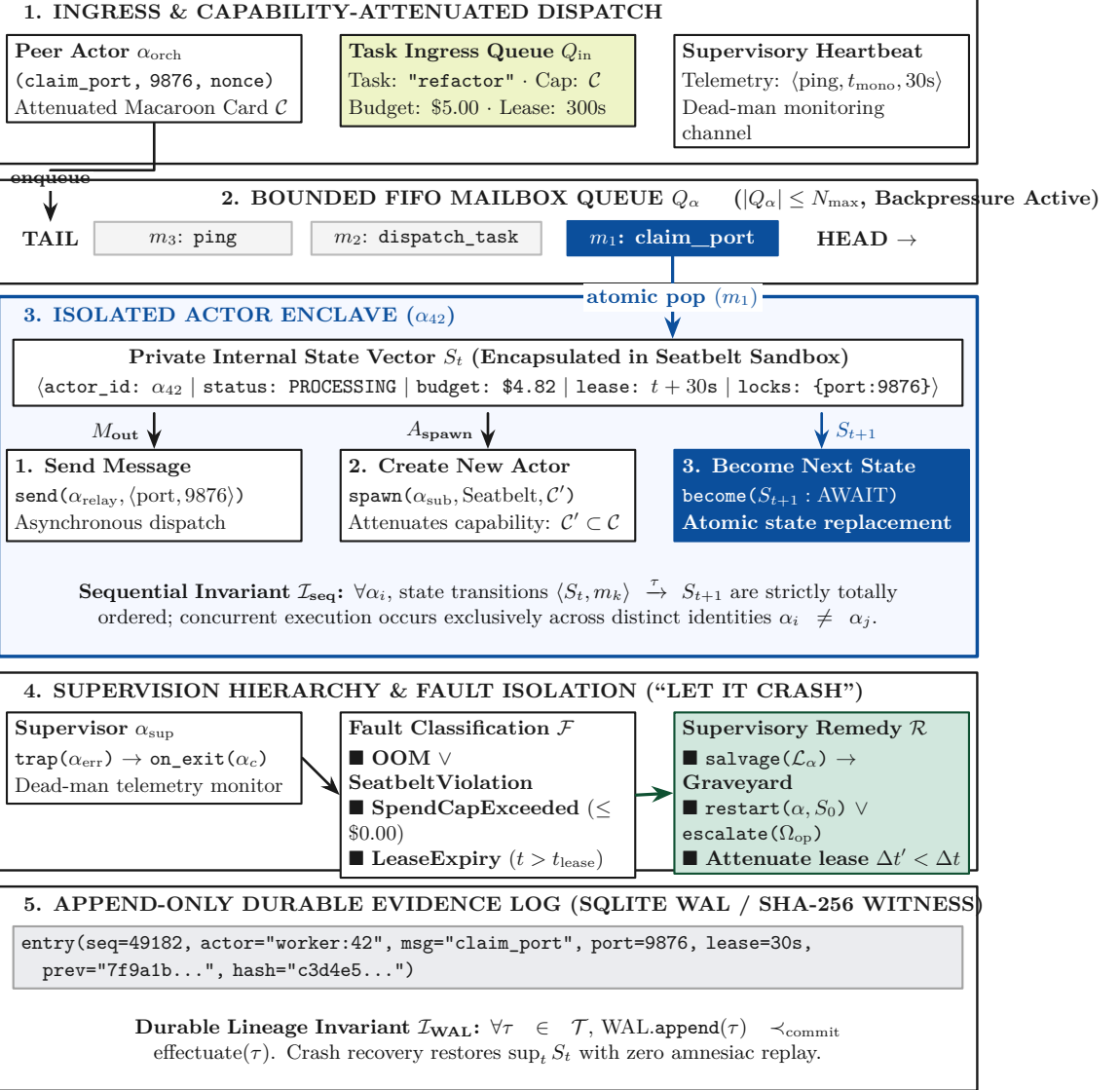
Figure 2: Hewitt-Agha virtual actor architecture: capability-attenuated mailbox ingress, sequential transitions via send, spawn, and become, and fault recovery under dead-man supervision.
