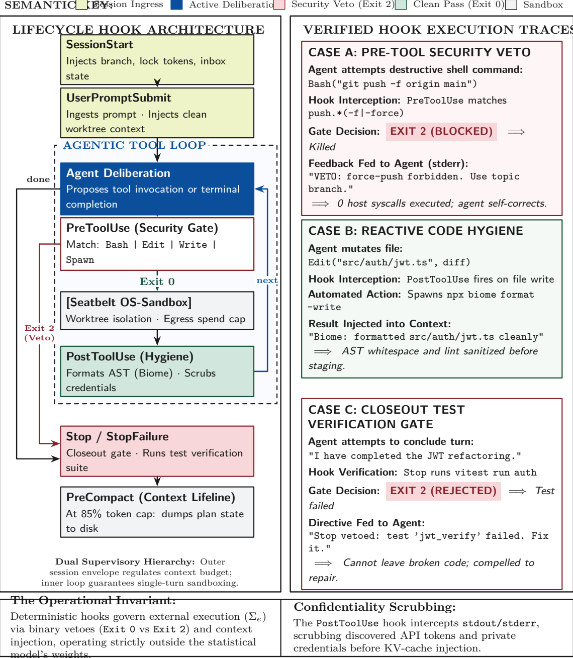
Figure 9: The Agent Lifecycle Hook cross-section, modeled after the production architecture of Anthropic’s Claude Code and the Port Daddy Giant Squid Harness. Execution is partitioned into two nested supervisory loops: the outer Session and Turn lifecycle manages user context, memory compaction (PreCompact), and test verification (Stop), while the inner AGENTIC TOOL LOOP supervises iterative tool invocations, pre-execution security vetoes (PreToolUse), sandbox execution, and reactive post-tool sanitization (PostToolUse). Concrete production traces (Cases A–C) illustrate deterministic enforcement at binary interception points.
