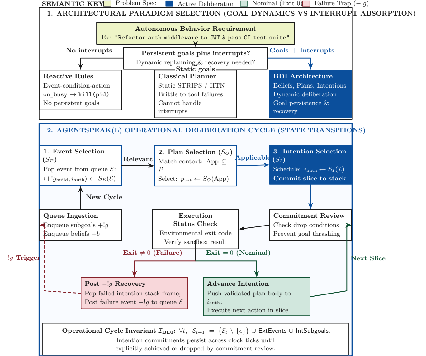
Figure 1: BDI execution flow and operational choice architecture, grounded in real-world software engineering workflows. Adapted from AgentSpeak(L) semantics [4], contrasting reactive rule triggers, static STRIPS-style planners, and dynamic BDI agents. The three core selection functions ( S_E for events, S_O for applicable plans, and S_I for intention stacks) arbitrate runtime goal scheduling, with explicit plan failure handling via the !g recovery event.
