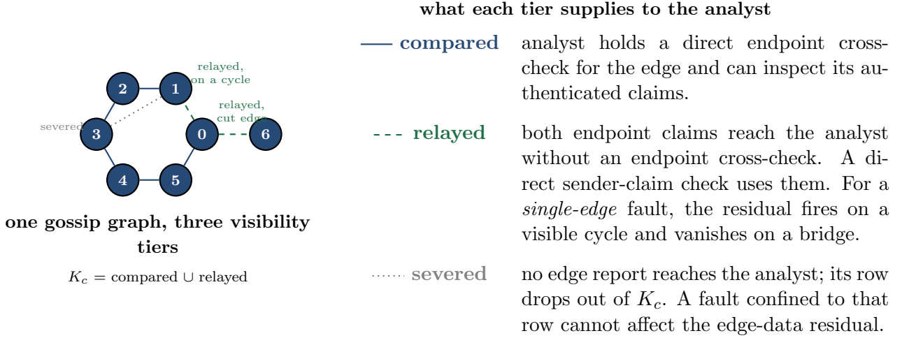
Figure 1: The three-tier observability contract — the tiers are properties of the analyst's evidence , not of the federation, and all three coexist on one topology. Left: one gossip graph wearing all three tiers — harborblue solid compared, seagreen dashed relayed, gray dotted severed; the compared-plus-relayed links are the visible subgraph K_c that the one-edge residual criterion uses. The severed link 1–3 is drawn as a chord. Right: the evidence supplied by each tier. The relayed tier already supplies both claims to an equal-information checker. The visible-cycle criterion describes the residual for one edge fault; it does not cover every one-sender split view. Figure 2 uses this same legend [internal, sheaf_harness_v2.py ].
