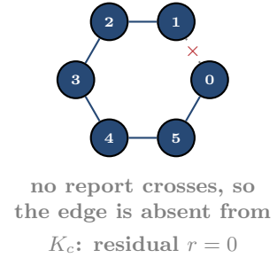
(c) C_6 , lie on a severed edge
