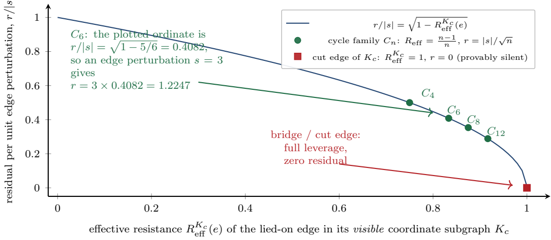
Figure 3: One-edge residual sensitivity is set by the visible topology and chosen Euclidean feature metric. The closed form plots residual per unit edge perturbation , r/|s| = \sqrt{1 - R_{\text{eff}}^{K_c}(e)} , against the effective resistance of the lied-on edge in its visible coordinate subgraph K_c — compared-plus-relayed links only, so severing a link on the edge’s cycle moves the point right, toward silence. The cycle family C_n sits at R_{\text{eff}}^{K_c} = \frac{n-1}{n} ; the marked C_6 point is the plotted ordinate 0.4082, which an absolute lie of s = 3 scales to the harness’s r = 1.2247 . The cut-edge corner R_{\text{eff}}^{K_c} = 1 is provable silence [verified; closed form exact on C_4 – C_{12} and 200 random graphs, sheaf_consistency_radius.py ].
