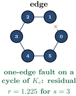
Figure 2: Regime diagram for the mechanism, in one legend with Figure 1 (harborblue solid compared, seagreen dashed relayed, gray dotted severed; the shipred \times marks the lied-on link, independently of its tier). (a) A single-edge fault on a relayed link in a visible cycle gives r = 1.225 for s = 3 . (b) The same fault on a relayed bridge gives r = 0 . (c) A severed edge has no row in K_c and cannot affect this residual. The relayed endpoint claims in (a) and (b) also permit direct sender-claim comparison when authenticated and snapshot-aligned. The figure states a one-edge residual criterion, not a unique detection advantage or a criterion for every split view [internal, sheaf_harness_v2.py].
