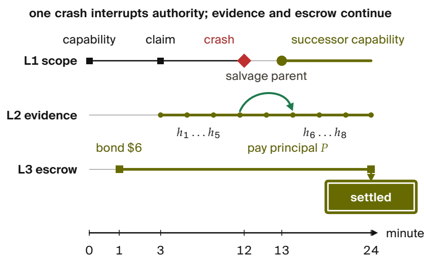
Figure 7.16. Three layers share one wall-clock axis. Process authority ends at minute 12 and a successor receives a new capability at minute 13. The evidence chain bridges the crash through a salvage-parent edge, while the pre-funded $6 escrow remains live until settlement at minute 24. The crash therefore disposes of identity without disposing of attribution or cleanup exposure. [internal]
