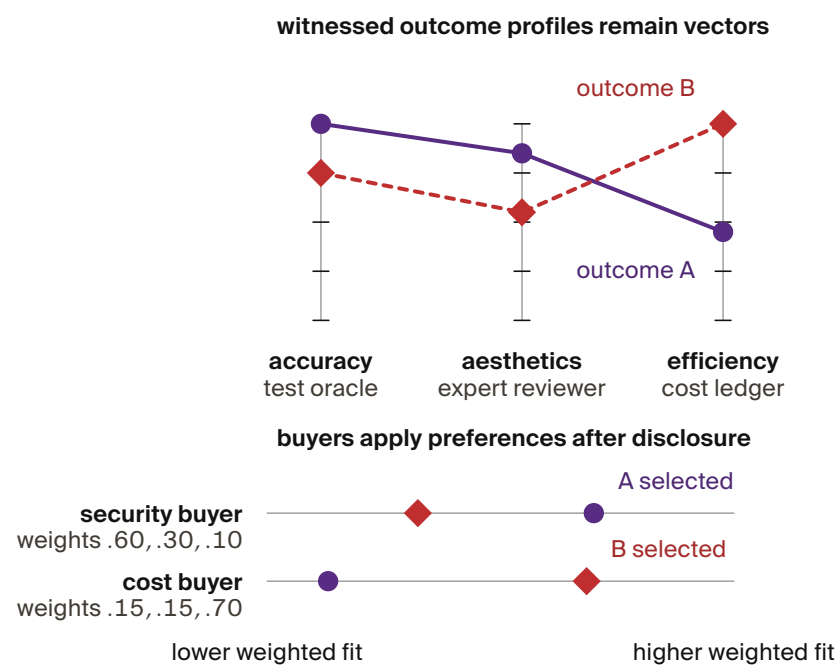
Figure 5.11. A favours accuracy and aesthetics; B favours efficiency. Different buyer priorities legitimately reverse the ranking. A universal average would erase that choice. [internal]
