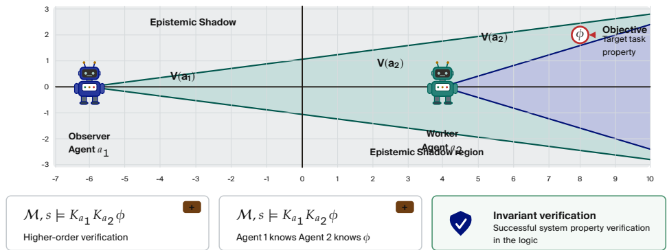
Figure 0.13: Dynamic Epistemic Observation Cones in Big Brother Logic (BBL) (Charrier et al., 2014). Directed vision cones formalize asymmetric visibility, epistemic shadows, and higher-order knowledge verification ( K_{a_1}K_{a_2}\phi ) in autonomous multi-agent systems. The supervisor maintains epistemic dominance over worker mutations, while sandboxed tenants operate within strict epistemic shadows, preventing side-channel data exfiltration.
