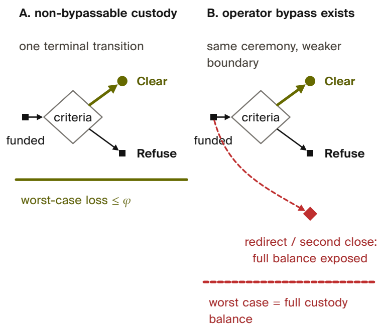
Figure 8.9. With a non-bypassable gate, recipient whitelist, and fee cap, custody closes only by payment or refund. Adding an operator-controlled escape exposes the entire balance, not merely the fee. [internal]
