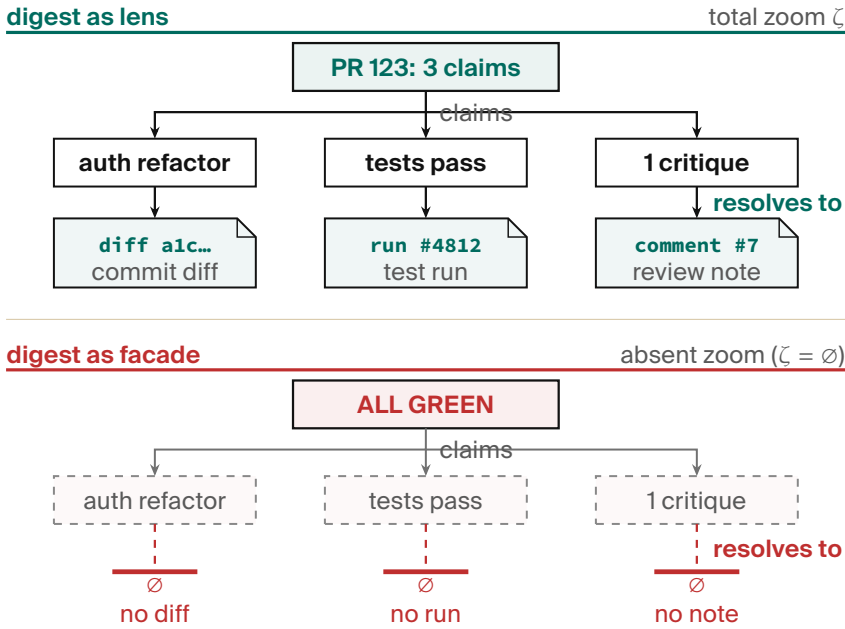
Figure 4.3. Two claim trees of identical shape. Top: the legible digest’s three named claims each resolve to one artifact — a diff, a test run, a review comment. Bottom: a same-shaped summary whose three claims resolve to nothing an operator can open. A safe summary is an index into evidence; a calm one that terminates early is a Potemkin digest, whichever claim count it advertises [internal].
