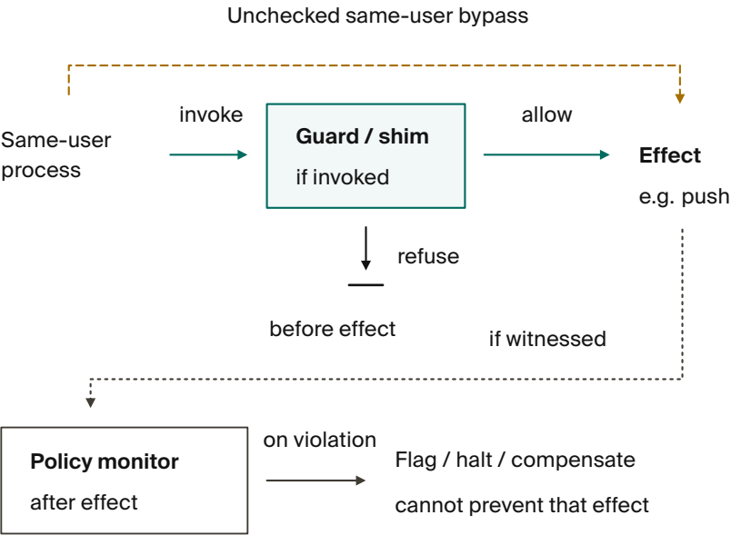
Figure 1.23. Refusal is not compulsory mediation. Grades are source-reported, not an independent runtime audit.
