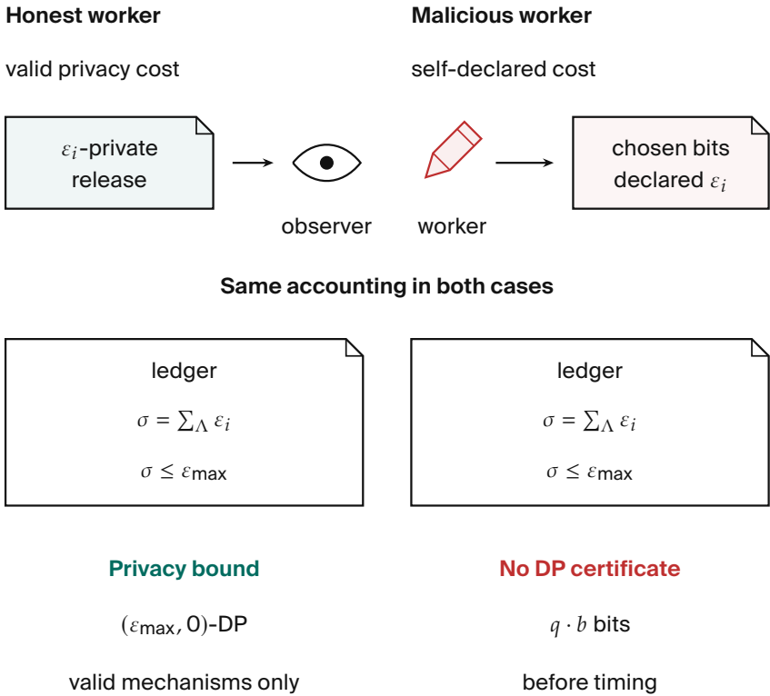
Figure 3.9. The same ledger conserves declared spend, not semantic privacy. DP needs valid mechanisms and complete mediation; q \cdot b bounds only the specified output channel before timing. [internal, §3.7]
