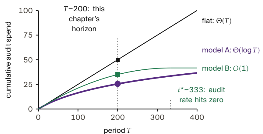
Figure 5.14. Model A's audit rate falls, but its cumulative bill has no finite ceiling. [verified, b2_tower.py, seed 20260816]
