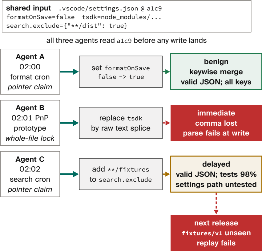
Figure 4.1. Three worked traces start from one settings.json revision. A keywise merge is benign; a raw splice fails immediately; a valid exclusion stays green until release replay exposes the hidden fixture. [internal, pedagogical counterexample]
