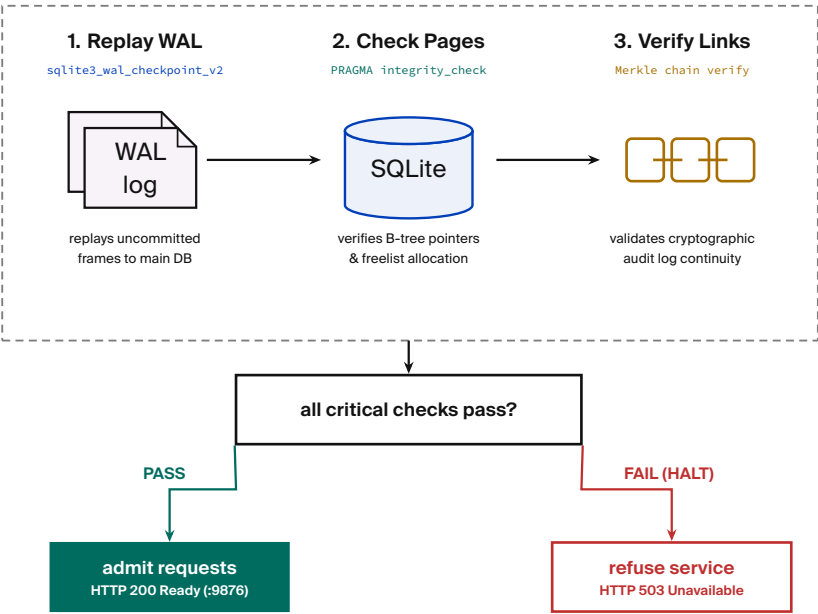
Figure 1.4. Three recovery mechanisms preceded admission. A failed critical check blocks service. The dashed group marks separate mechanisms, not a completed shared recovery invariant.
