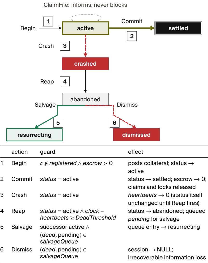
Figure 7.13. A crashed session becomes abandoned after the reaping threshold, then is salvaged or dismissed. File claims only inform; they do not exclude another claimant. [internal, BondedCommons.tla]
