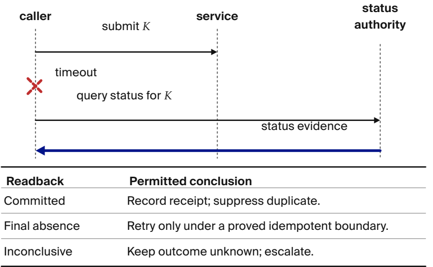
Figure 1.19. A timed-out external operation leaves its effect unknown. The caller queries an operation-specific authoritative status before deciding whether to record a receipt, retry under a proved idempotent boundary, or preserve an unresolved outcome. An absence result permits retry only when the authority excludes a late commit for K ; the drawing does not make unbrokered delivery exactly once [internal].
