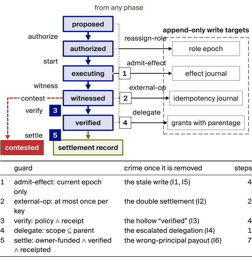
Figure 1.20. Five guards protect the work-unit lifecycle. In the two-principal model, all 536 reachable states satisfy six invariants; removing any guard exposes the counterexample listed below. [internal, c0_workunit.py]
