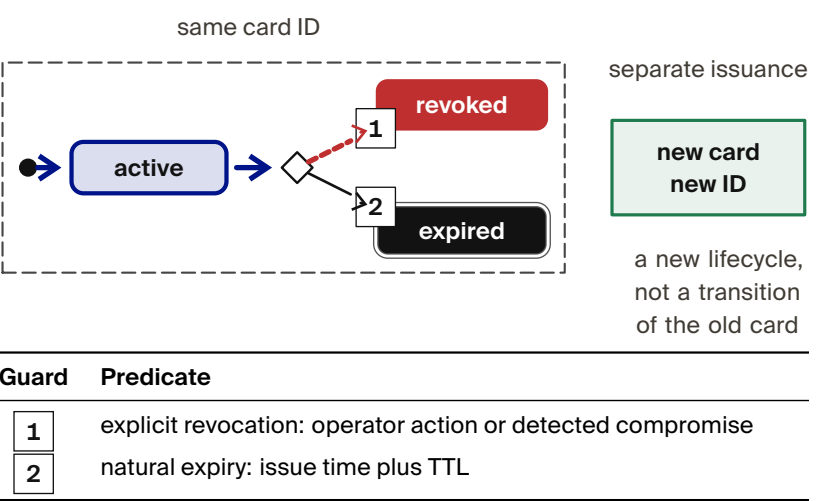
Figure 2.8. A UML state machine gives one card ID exactly two guarded terminal exits. Fresh issuance is shown separately, with no outgoing path from the revoked or expired card. [internal]
