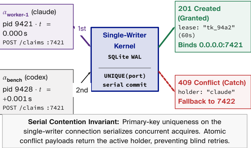
Figure 1.7 draws the two lanes converging on that one commit point and the two outcomes.
