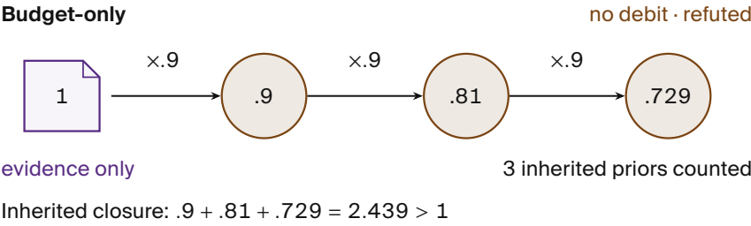
Figure 5.5. Transfer spends each source balance; an undebited copy retains it. The first row counts inherited priors, the others spendable balances.
