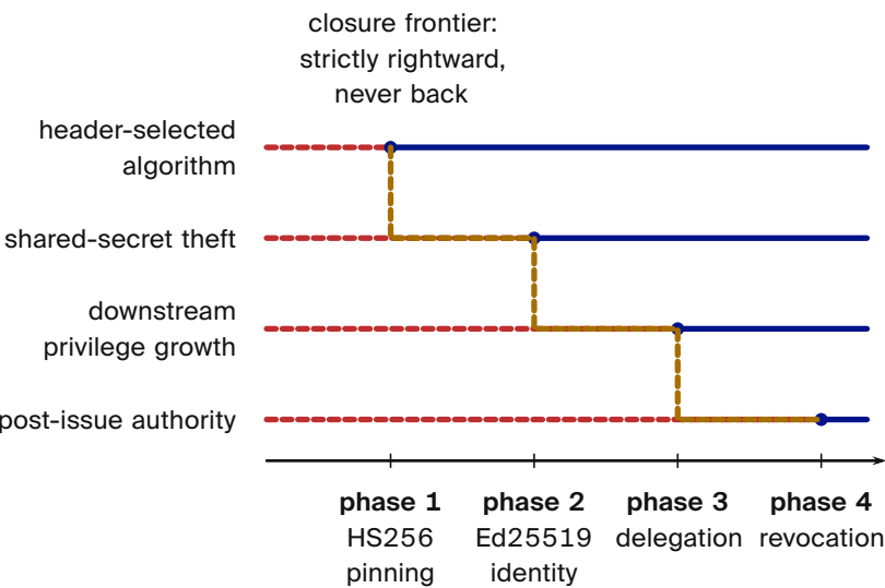
Figure 2.1. Each phase adds a check without removing earlier checks. The marked transition closes the named threat; later phases preserve that closure. [internal, Table 2.1]
