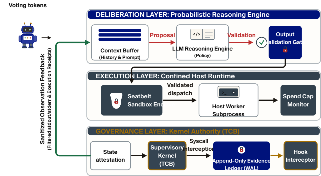
Figure 0.18: The Closed Agentic Architecture Loop. Three architectural tiers separating probabilistic deliberation from deterministic kernel coordination: (1) Probabilistic Deliberation Layer (LLM reasoning and planning); (2) Confined Execution Layer (sandboxed host containers and tool execution); and (3) Deterministic Governance Layer (single-writer SQLite WAL, capability verification, and tamper-evident Merkle attestation).
