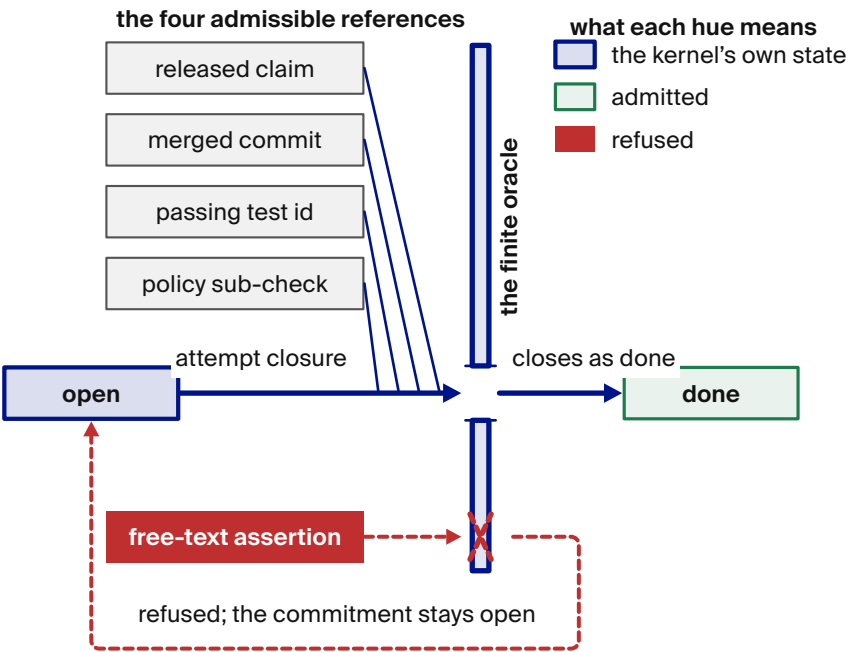
Figure 1.16. Closure requires a supported evidence reference rechecked by the daemon. Free-text assertions leave the commitment open; scope policy, not the agent, supplies its deadline. [internal]
