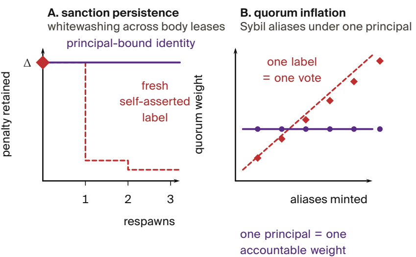
Figure 5.8. Binding identity to a principal preserves sanctions across restarts and prevents aliases from multiplying quorum weight. This protection is local to one trusted domain, not cross-operator attestation. [internal]
