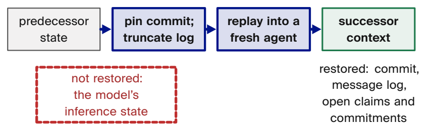
Figure 1.18. Proposed replay restores recorded inputs and durable task state, not hidden model inference state. Completeness remains unestablished; OP-4 is not closed. [internal]
