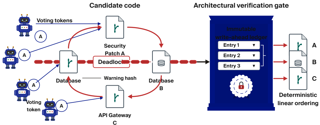
Figure 0.14: Arrow's Impossibility Theorem in Autonomous Multi-Agent Consensus. Kenneth Arrow (1951) demonstrated that with |A| \geq 3 , no ordinal preference aggregation function can simultaneously satisfy Unrestricted Domain (U), Weak Pareto (P), and Independence of Irrelevant Alternatives (IIA) without degenerating into a Dictatorship (D). In multi-agent systems, naive voting induces Condorcet cycles ( A > B > C > A ). Port Daddy avoids ordinal voting cycles by using cardinal utilities, bonded escrow, and VCG clearing.
