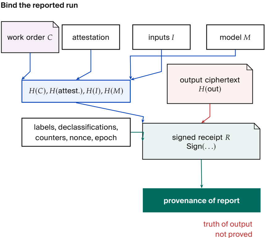
Figure 3.4. Hashes and the signature bind the recorded work order, evidence, inputs, model, policy state, and released ciphertext. The receipt proves what was reported, not that the output is true.
