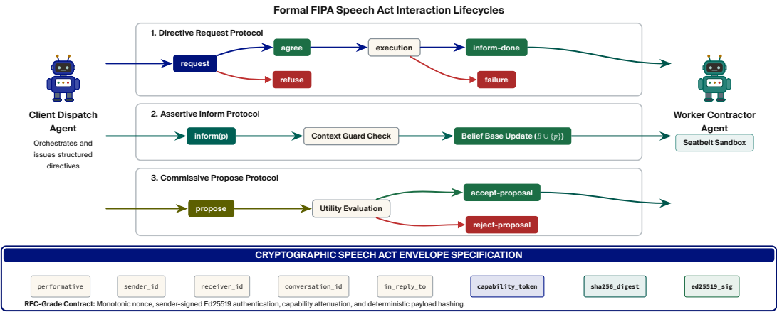
Figure 0.11: FIPA-00037 Communicative Speech Act State Transition Machine. Grounded in practical software engineering payloads. Top: Directive request lifecycle executing an atomic database migration under lock arbitration. Middle: Assertive inform directly mutating an agent’s belief base. Bottom: Commissive propose negotiating an SLA for canary deployment routing. Every envelope carries cryptographic sender/receiver verification, monotonic capability tokens, and explicit conversation correlation IDs.
