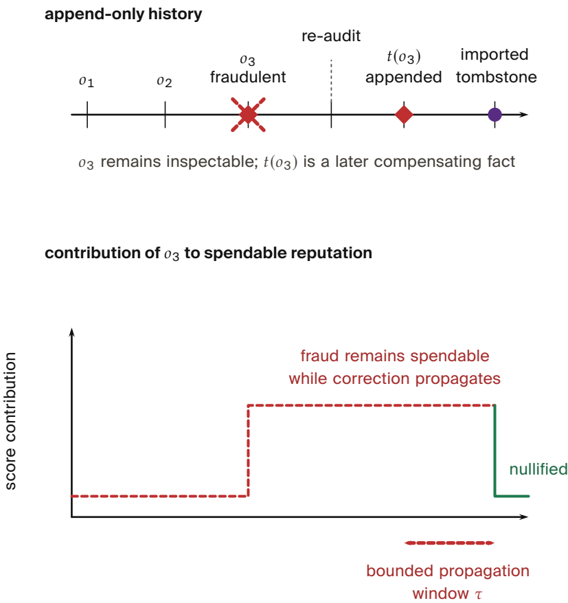
Figure 5.16. A tombstone removes a fraudulent contribution from future scoring without erasing history. Importing harbors remain exposed until it arrives; \tau measures that convergence interval. [internal]
