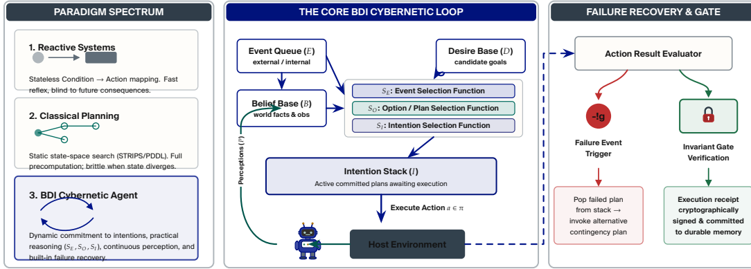
Figure 0.9: BDI Execution Flow and Operational Choice Architecture. Grounded in real-world software engineering workflows, adapted from AgentSpeak(L) semantics (Bordini et al., 2007). Contrasting reactive rule triggers, static STRIPS-style planners, and dynamic BDI agents. The three core selection functions ( S_E for events, S_O for applicable plans, and S_I for intention stacks) arbitrate runtime goal scheduling, with explicit plan failure handling via the \neg!g recovery event.
