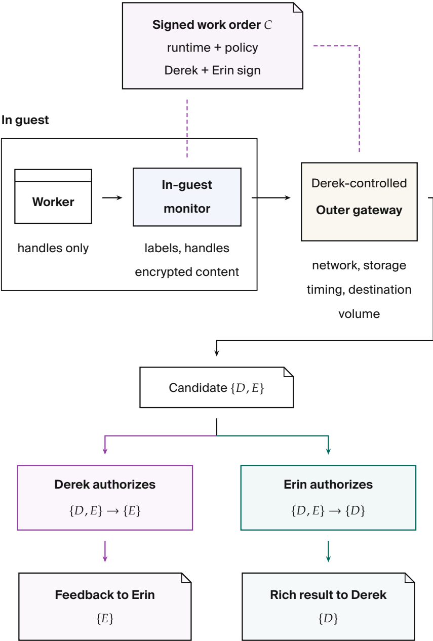
Figure 3.5. Each owner authorizes removal of their own restriction. Dashed links bind controls to the signed work order; solid arrows carry outputs. Proposed control flow; public receipt omitted.
