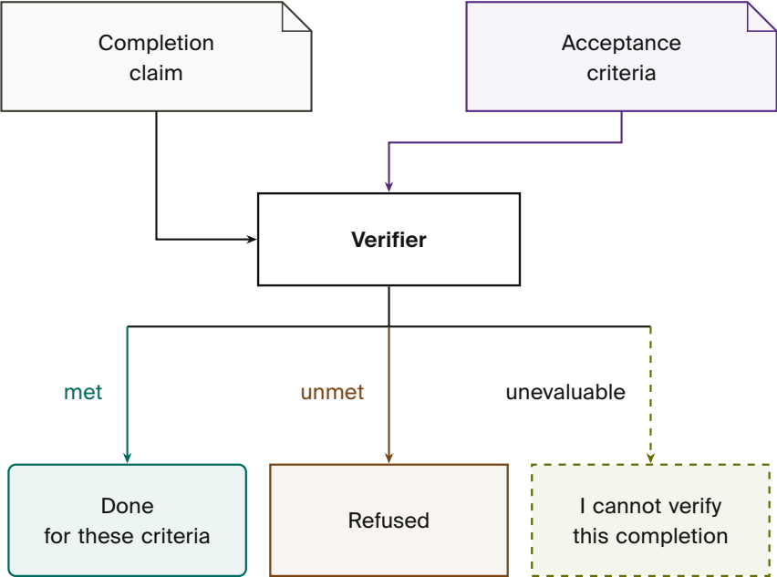
Figure 4.7. Vision: a proposed authority-side rule, not implemented enforcement or a guarantee of universal correctness. Passing it still leaves any omitted requirement unchecked.
