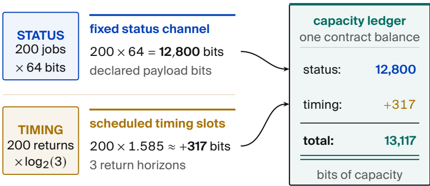
Figure 3.14. For 200 jobs, fixed status plus three return slots yields about 13,117 bits of adversarial capacity. The capacity ledger accounts for both explicit payloads and discrete timing horizons without conflating their channels. [hand-derived; Exercise 3.12]
