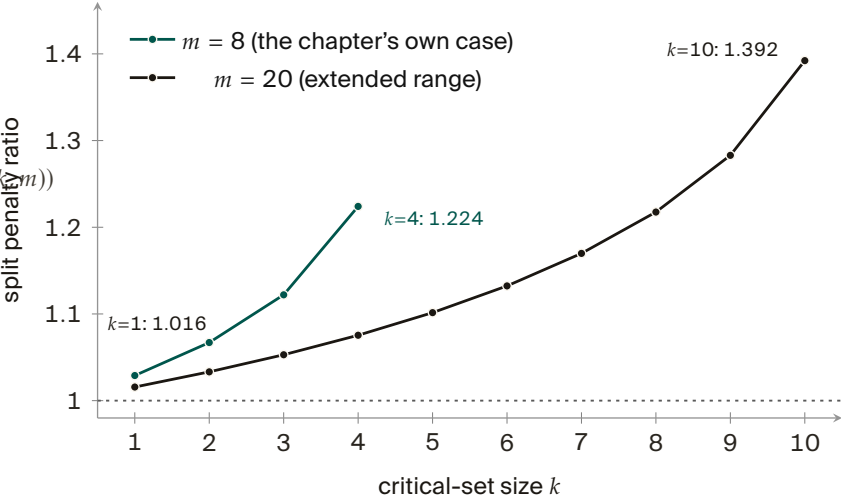
Figure 4.16. The joint zero-miss digest’s penalty over twice the single-reader floor, \text{Floor}(N, 2k, m)/(2 \text{Floor}(N, k, m)) at N=60 , plotted over its whole domain rather than the four hand-worked points alone. Both plotted ratios exceed the dashed 1.0 parity line and rise monotonically. For one union selection under a shared m -open budget, the joint floor exceeds twice the single-set floor: 1.392\times at m=20, k=10 and 1.224\times at m=8, k=4 . This is a selection-budget comparison, not a requirement for separate models or stores. [internal; analytic]
