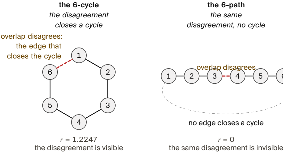
Figure 8.7. Cycle versus cut on six harbors, numbered 1 to 6. The same one-edge perturbation on one overlap is placed on the cycle C_6 and on the path P_6 . On the cycle the disagreeing edge closes a visible cycle and the consistency radius is r = 3(1 - 5/6)^{1/2} = 1.2247 ; on the path no edge closes a cycle and r = 0 , so the one-edge residual is exactly governed by the visible-cycle condition. Authenticated endpoint claims can also be compared directly in either topology. [verified; sheaf_consistency_radius.py, seed 20260816] Samson Abramsky and Adam Brandenburger. The operational-sheaf-theoretic approach to contextuality and non-locality. New Journal of Physics , 13(11):113036, 2011.
