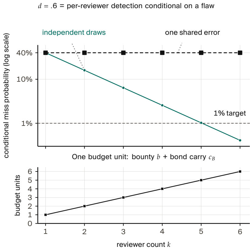
Figure 6.9. In this analytic model, more independent reviewers reduce miss probability; perfectly shared outcomes do not. The lower panel is reserved budget, not realized payout.
