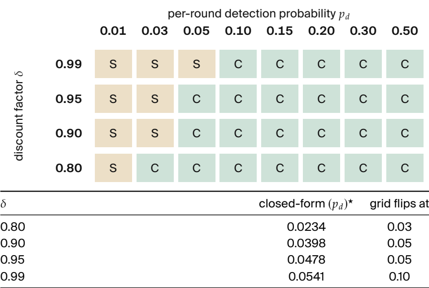
Figure 7.12. S means the cartel sustains; C means it collapses. Every simulated boundary lies within one tested grid step of the closed-form threshold (§7.6.5.10). Each configuration uses 5,000 trials, 200 rounds, and three colluders. [verified, proofs/bonded/pareto/simulation-cartel.mjs]
