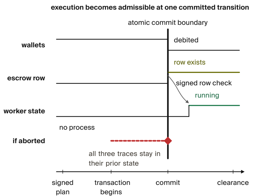
Figure 6.2. Proposed admission order: requester bounty and provider bond are reserved together. The worker waits for the reservation receipt. The signed ceremony and enforced gate are not yet complete. [internal]
