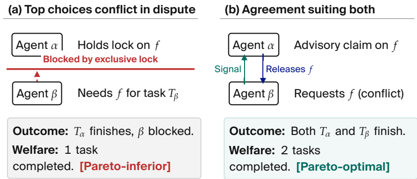
Figure 7.5. Precautionary locks versus advisory claims. In panel (a), agent \alpha 's decisive lock on an unneeded file f aborts agent \beta 's task T_\beta . In panel (b), advisory notification lets \alpha release f , achieving the Pareto-superior outcome where both tasks succeed.
