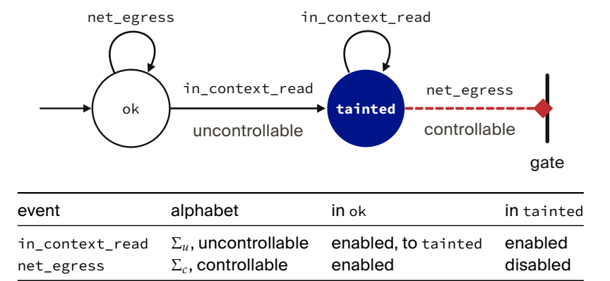
Figure 1.14. Reading a secret records taint; it is never refused. Afterward the policy blocks mediated network egress, while leaving uncontrollable events enabled. [internal, b3_controllability.py]
