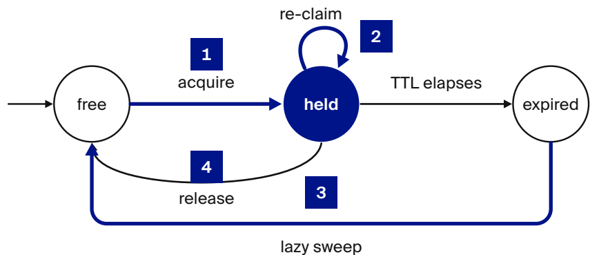
Figure 1.5. The guarded claim lifecycle as a finite-state machine. Acquire is a single atomic insert against a SQLite uniqueness constraint; re-claim and release are idempotent; expiry moves a claim to expired , from which the next read lazily sweeps it back to free . There is no queued state: losing callers receive 409 Conflict and must manage their own backoff. [internal, alg:acquire]
