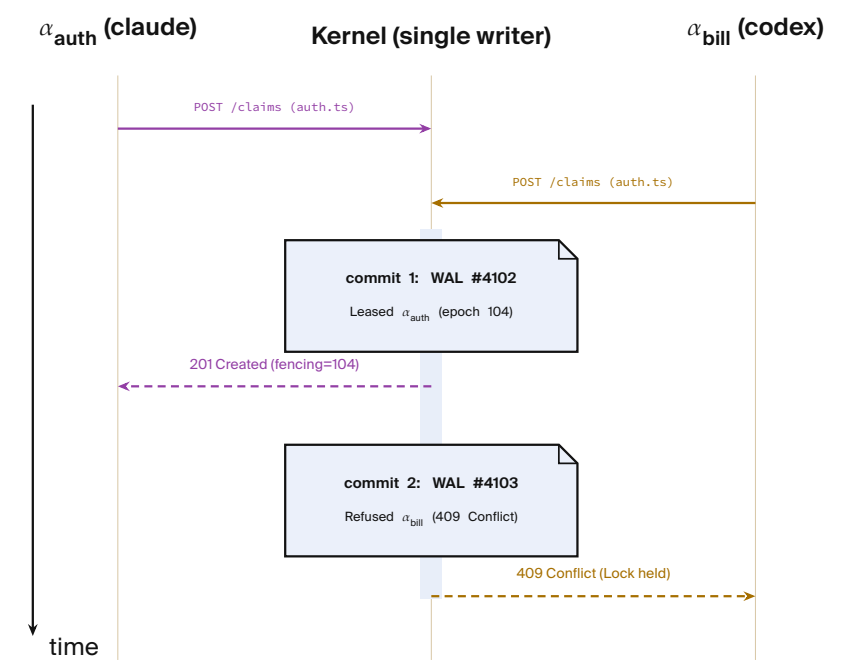
Figure 1.2. Both requests arrive before the first commit. The writer orders their records and replies after each commit. This sequence assumes one writer; it does not establish power-loss durability.
