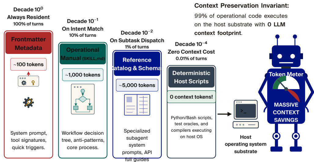
Figure 0.15: Progressive Disclosure of Skills Across Contracting Logarithmic Decades. Capability activation frequency contracts across decades ( 10^0 to 10^{-4} ). By partitioning capabilities from static frontmatter metadata down to host-executed scripts and formal schemas consuming zero LLM context tokens, context consumption contracts exponentially with task specialization.
