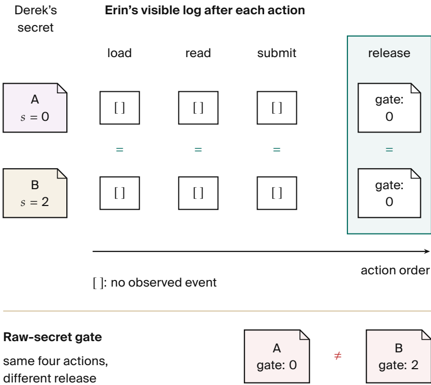
Figure 3.6. Parity hides the difference between secrets 0 and 2; a raw-secret release exposes it. Reported model check: four secrets, depth 7, not unbounded executions. [internal, c1_noninterference.py]
