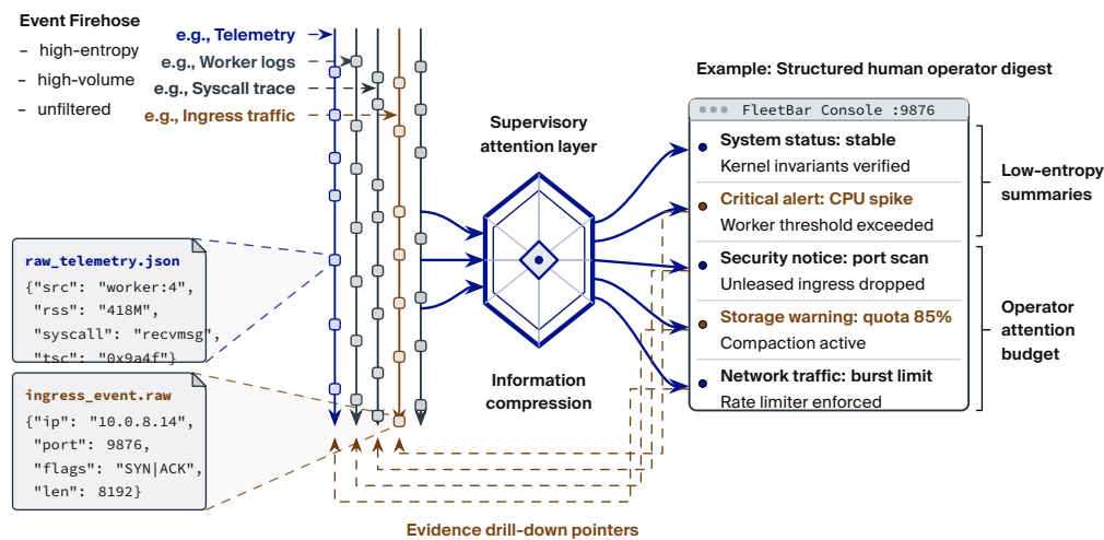
Figure 0.4: Proposition 4 Mechanics: Information Cost and Evidence Drilling. Supervisory digests operate as reversible, low-entropy projections indexed into an immutable Merkle evidence log. An operator can drill down with zero friction from high-level fleet status down to exact execution receipts and byte-level syscall traces.
