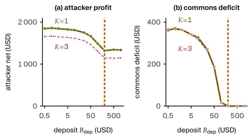
Figure 7.10. Reimbursing the commons does not eliminate attacker profit. Across the tested deposits, one or three Sybil identities remain profitable because slashing is capped by coverage. [verified, proofs/bonded/pareto/simulation-sybil.mjs]
