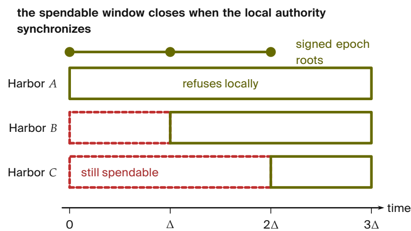
Figure 8.4. Revocation reaches each harbor separately: here A refuses immediately, B after \Delta , and C after 2\Delta . A partition can extend staleness without bound. [internal]
