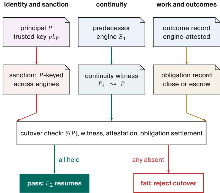
Figure 5.10. A migration accepts only with principal-scoped sanctions, a continuity witness, engine-attested outcomes, and closed or escrowed obligations. The successor receives a continuing record, not a clean slate. [internal; schematic]
