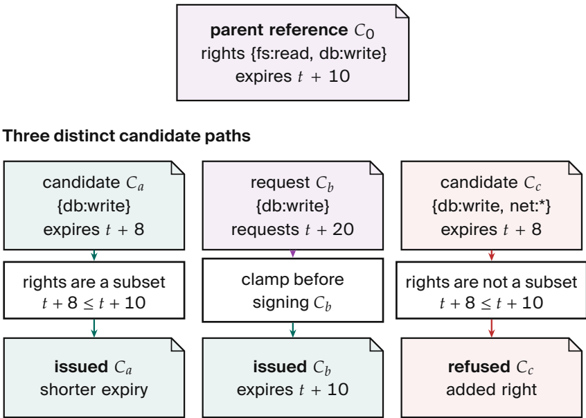
Figure 2.2. Every hop checks a rights subset and an expiry bound. A child may inherit its parent’s expiry when a longer lifetime is requested; it may never gain a new right.
