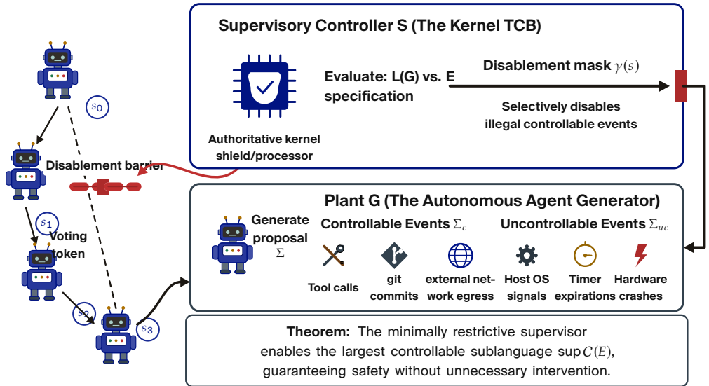
Figure 0.17: Ramadge-Wonham Discrete-Event Supervisory Control in Multi-Agent Swarms. Uncontrolled swarm execution G is restricted by supervisory controller S to enforce safe language K \subset L(G) . Controllable tool events \Sigma_c (file writes, process spawns, network requests) that violate mutual exclusion or spend caps are disabled by the supervisor, guaranteeing system-wide safety invariants.
