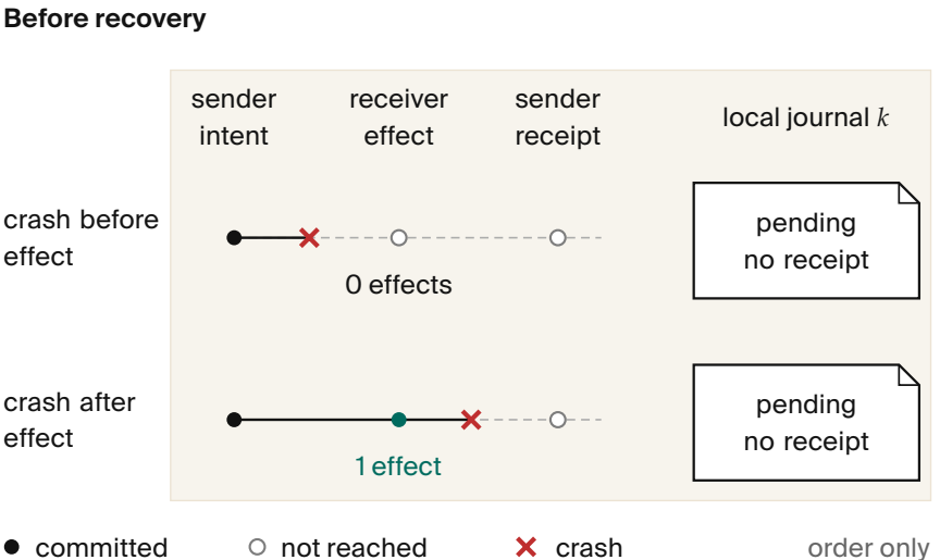
Figure 1.9. A missing receipt does not reveal whether the effect happened. Twelve local SQLite cases, not a Port Daddy test. Receiver deduplication here atomically retains the key, payload, effect and receipt; a sender-side key alone does not supply that contract. [Local fixture, receipt_gap_experiment.py.]
