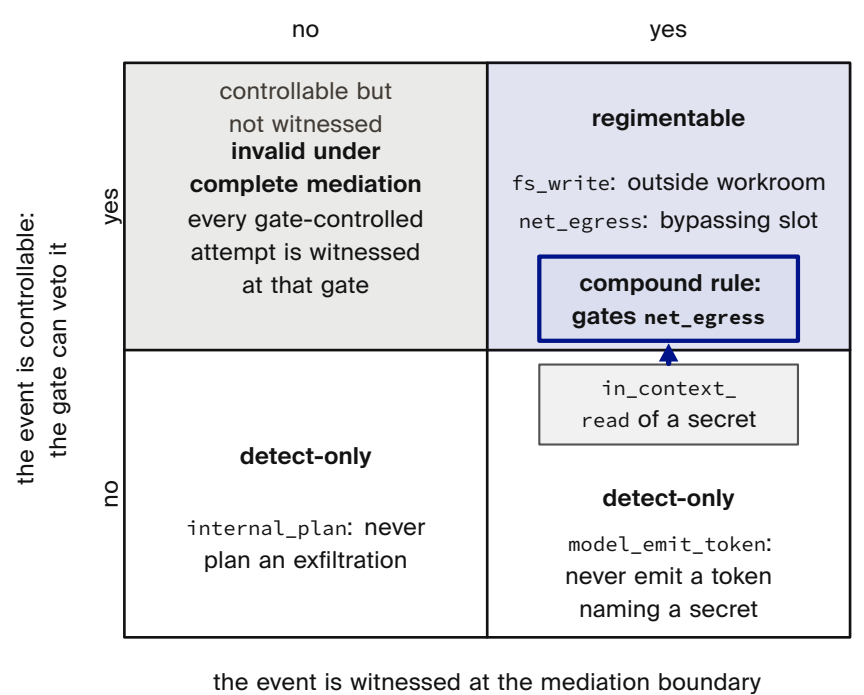
Figure 3.8. Room events on controllability × witnessing. Complete mediation makes the upper-left cell invalid: every gate-controlled event is witnessed. The compound rule watches the read, then vetoes net_egress. [internal, b3_controllability.py]
