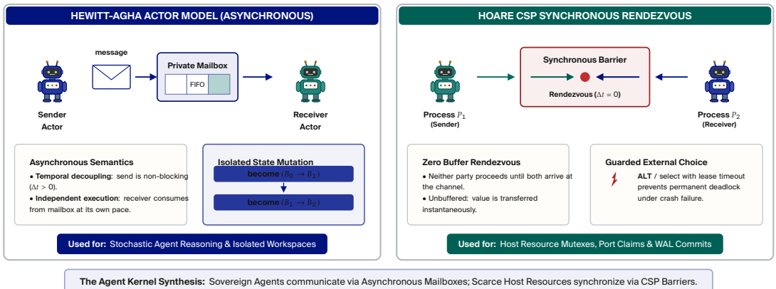
Figure 0.10: Concurrency Foundations for Multi-Agent Operating Kernels. Synthesizing Hewitt-Agha virtual actor isolation (asynchronous mailboxes, capability tokens, and become state transitions) with Hoare's Communicating Sequential Processes (synchronous rendezvous barriers, \Delta t = 0 , and guarded external choice with lease timeouts). Sovereign actors deliberate in isolated sandboxes, while physical host resource contention (TCP ports, SQLite WAL writes, git locks) is arbitrated via synchronous CSP rendezvous.
