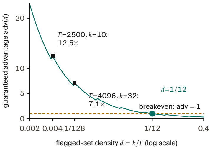
Figure 4.14 plots the guaranteed advantage \text{adv}(d) itself against flagged-set density, marking the crossing at d = 1/12 alongside the chapter’s own F=2500, k=10 and F=4096, k=32 configurations.
