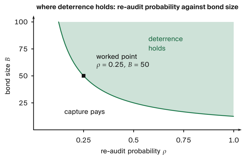
Figure 5.15. Deterrence requires \rho dB \geq G . For G = 10, d = 0.8, B = 50 , the threshold is \rho = 0.25 ; lower audit probability makes capture profitable. [internal; closed form]
