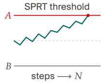
Wald stopping boundary: Sequential ratio walk with thresholds A, B .
