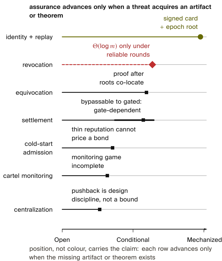
Figure 8.2. Evidence differs by threat. Identity and replay have concrete artifacts; revocation and settlement depend on stated connectivity and custody assumptions. Admission, cartel monitoring, and centralization remain open. [internal]
