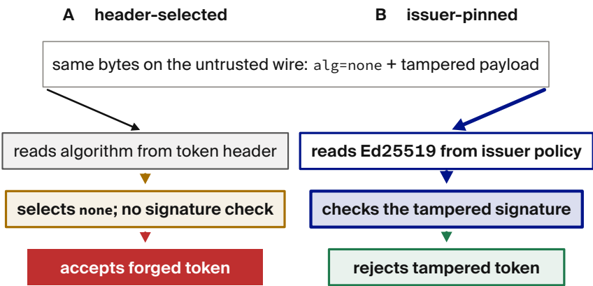
Figure 2.3. Aligned security traces hold the wire bytes constant and vary only the source of algorithm authority. Header selection reaches acceptance without a signature check; issuer pinning forces Ed25519 and rejects the same tampered token. [verified, v1_refined.pv]
