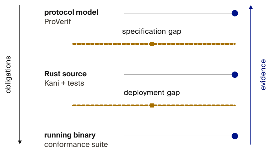
Figure 2.9. Obligations descend from model to source to binary; tool evidence returns upward. The two correspondence gaps still require human justification. [internal, Table 2.2]
