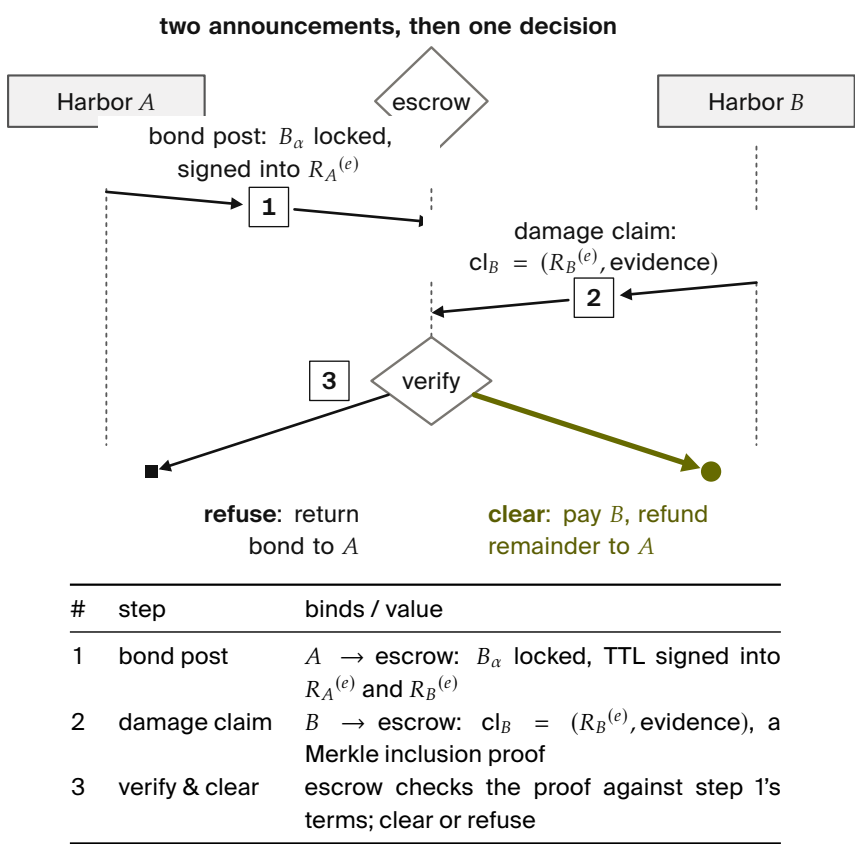
Figure 8.11. Posting a bond and announcing damage do not settle it. Escrow checks the proof against the signed conditions, then makes one terminal decision: clear or refuse. [internal]
