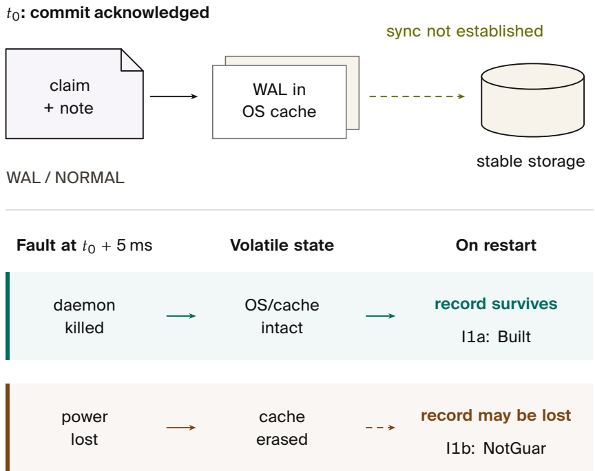
Figure 1.3. With OS and database/WAL state intact, restart recovers a process-crash commit; power loss can erase an unsynchronized commit. The five-millisecond interval is illustrative.
