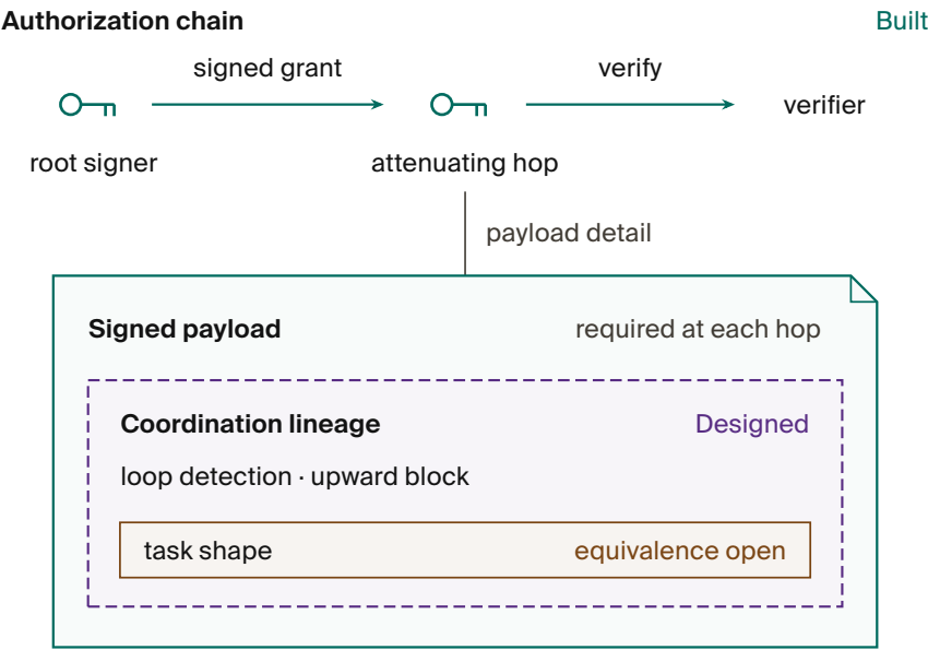
Figure 1.11. The designed coordination lineage must be carried inside each signed authorization hop. Authenticating its bytes does not establish semantic task equivalence.
