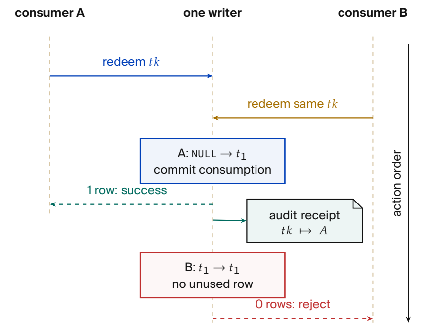
Figure 7.15. Overlapping requests still produce one consumption. A wins this illustrated schedule; either caller can win. SQL is simplified: authentication and expiry checks are omitted.
