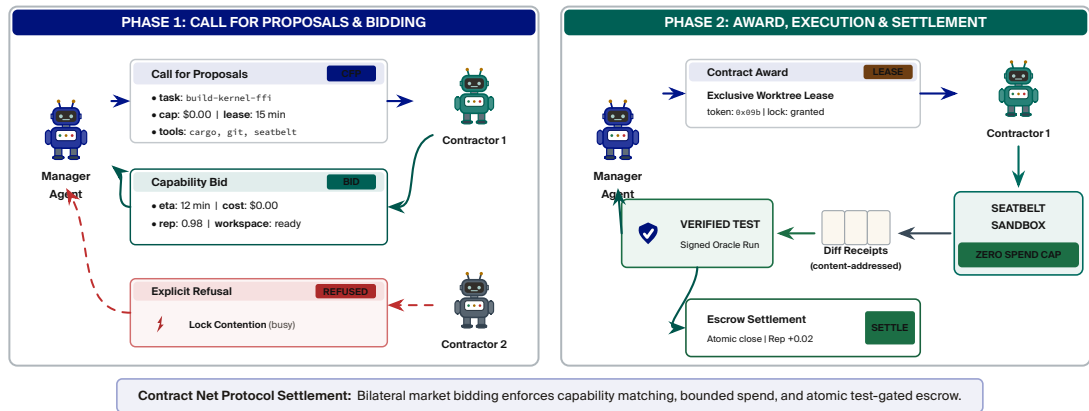
Figure 0.12: Contract Net Protocol (CNP) Task Allocation Lifecycle and Settlement Under Kernel Confinement. Grounded in Reid Smith’s (1980) bilateral market protocol. Phase 1 (left): Manager agent broadcasts a Call for Proposals (CFP) with task specification and spend cap; eligible contractors evaluate tool capacity and submit bids, or return explicit refusals under lock contention. Phase 2 (right): Winning contractor receives an exclusive worktree lease (0x09b), executing inside a Seatbelt sandbox under a zero-spend cap. Escrow funds unlock strictly upon presentation of signed git commit hashes and cryptographic test run receipts.
