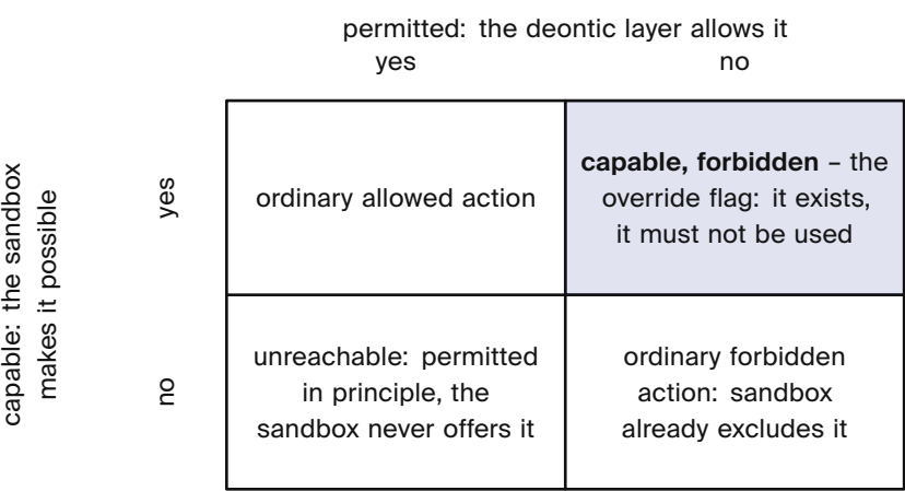
Figure 1.12. Capability and permission are independent. The shaded case is possible but forbidden—the state a collapsed vocabulary cannot express. [internal]
