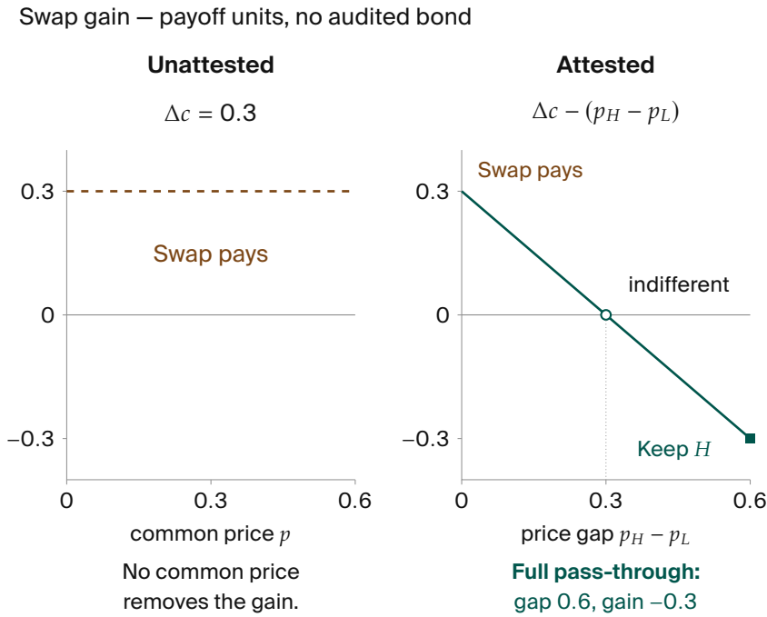
Figure 5.9. Attestation changes which price can deter substitution; it does not guarantee the price gap. Analytic example: \theta_H = 1 , \theta_L = 0.4 , c_H = 0.5 , c_L = 0.2 (Theorem 5.6.8).
