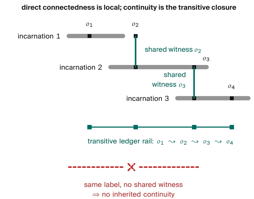
Figure 5.3. Parfitian continuity is an overlap chain, not permanent connectedness.
