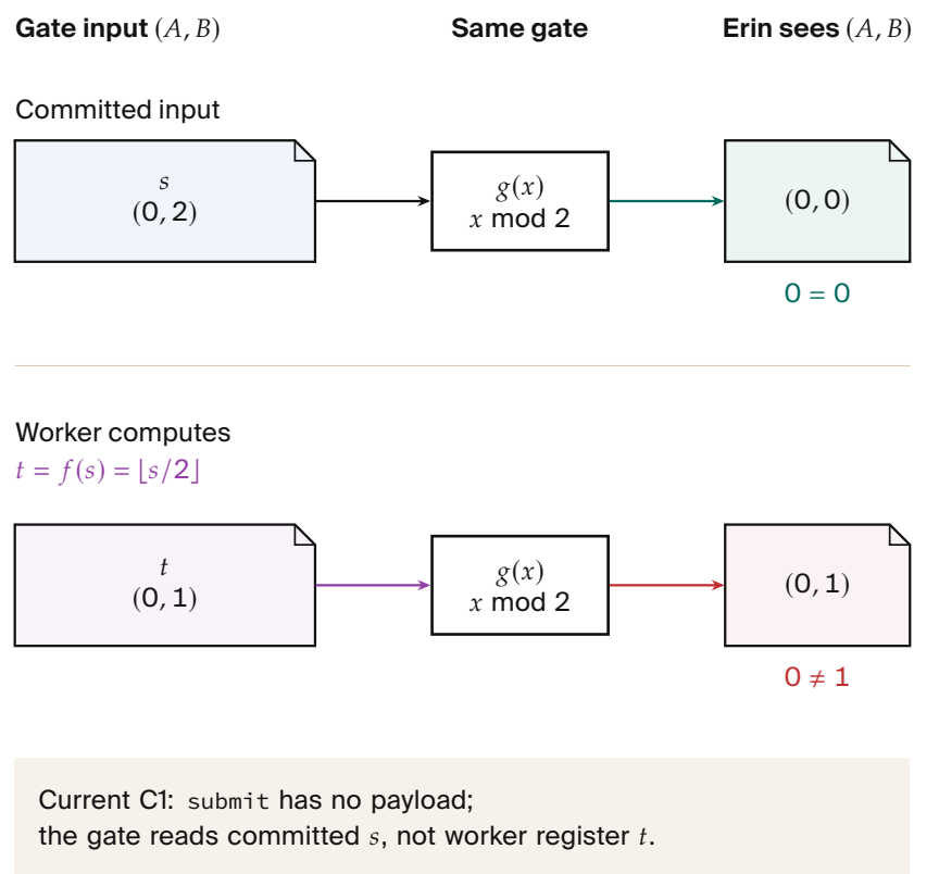
Figure 3.7. The gate is unchanged; the worker changes its argument and reveals a distinction the original parity release hid. This arithmetic example is outside C1's committed-input model. [internal; Exercise 3.4]
