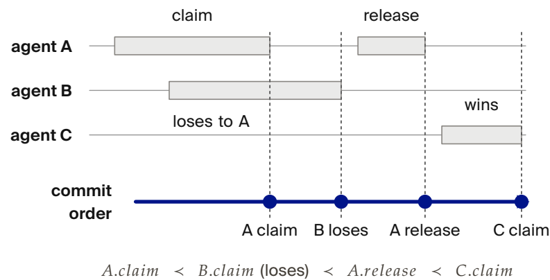
Figure 1.21. Overlapping requests receive one commit order: A claims, B loses, A releases, C claims. Theorem 1.10.3 states the five assumptions this ordering requires. [internal]
