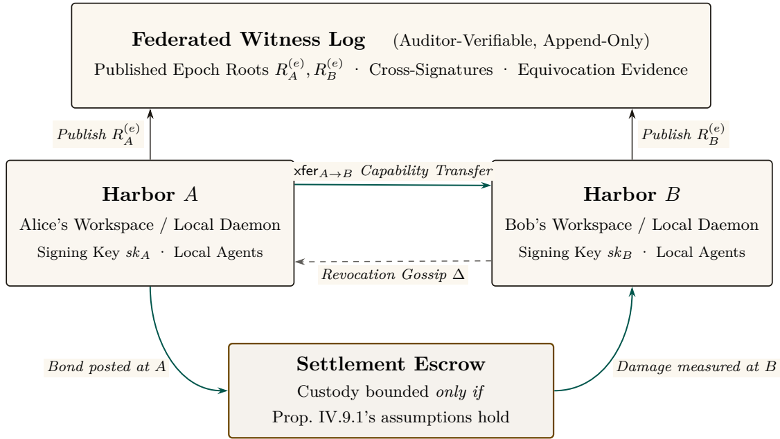
Figure IV.7: The Federated Harbor as a four-element gestalt. Neither harbor is a root of authority for the other. The witness log above provides shared correlation: each harbor publishes its signed epoch root, enabling decentralized equivocation detection. The settlement escrow below is structurally bounded conditional on a non-bypassable custody mechanism (§IV.9.2); 2-of-3 threshold signing is one candidate, and this paper does not establish that condition for a deployed system. The solid teal arrow denotes the capability transfer ceremony (§IV.8); the dashed line denotes epidemic revocation gossip (§IV.9.3).
