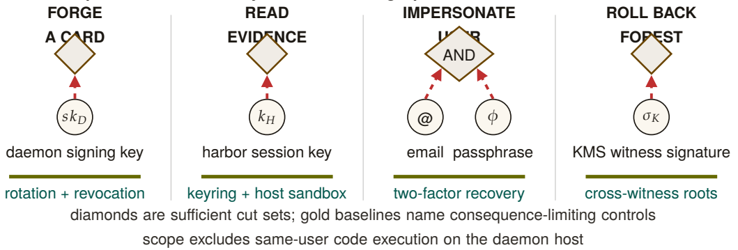
Figure 7.7: The custody theorem has four small attack cut sets rather than one undifferentiated trust boundary. Card forgery, evidence decryption, and forest rollback each have one sufficient secret; user impersonation is the sole conjunctive failure and requires both email and passphrase. The gold baselines name the consequence-limiting control for each cut. Same-user code execution remains outside the theorem because that adversary can read every secret available to the user process.
