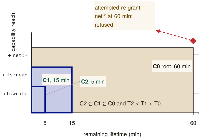
Figure 2.2: Nested rectangles for the capability envelope C_0 (root, 60 min), C_1 (15 min) and C_2 (5 min): each child rectangle sits strictly inside its parent on both axes. The amber datum is an attempted re-grant of \text{net}:* at the full 60-minute root lifetime, outside C_0 on the capability axis; the verifier refuses it because attenuation is conjunctive on rights and time together, not a trade between them. [internal]
