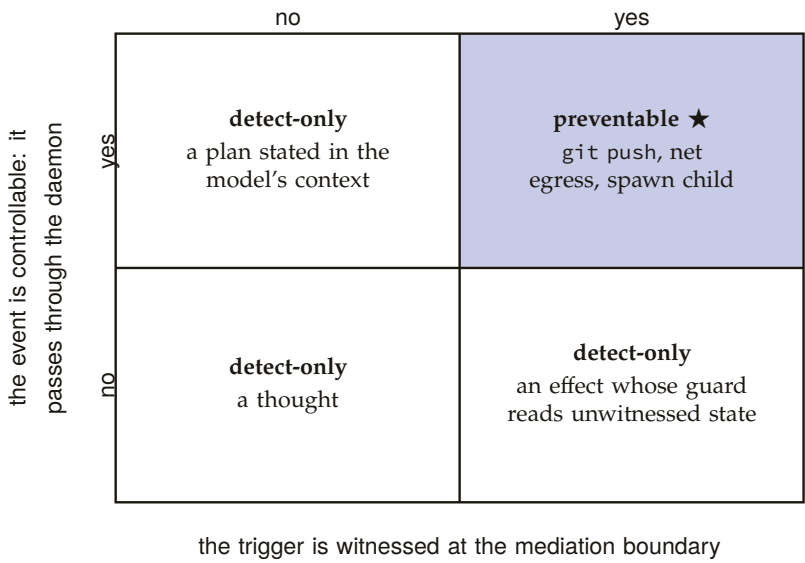
Figure 1.8. Preventable is one cell, not a spectrum. An event is preventable exactly when it is controllable (top row) and its trigger is witnessed at the mediation boundary (right column): the shaded cell, marked ★ and tied to Theorem 1.8.3. Every other combination is detect-only. Column membership reproduces from the checker [internal, b3_controllability.py]; row membership is by inspection of each trigger.
