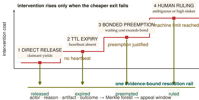
Figure 7.2. Dispute resolution is an escalation staircase. The system first offers a zero-coercion exit, then waits for the claimant’s TTL, then permits priced preemption, and reaches dispute path judgment only after the machine-readable options are exhausted. Every station can terminate the dispute, and every termination descends to the same evidence rail. Escalation therefore changes the decision cost and decision-maker without discarding the record needed for appeal.
