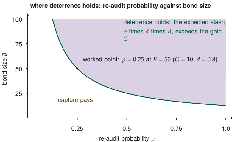
Figure 5.10. The deterrence frontier of the re-audit tower. A grader is deterred from selling a grade when the expected slash, re-audit probability \rho times detection rate d times bond B , exceeds the one-shot gain G ; the frontier is \rho B = G/d , drawn for G = 10 and d = 0.8 . The worked point of this section, B = 50 , sits on the frontier at the threshold \rho = 0.25 : any lower audit rate at that bond, or any smaller bond at that rate, lies where capture pays.
