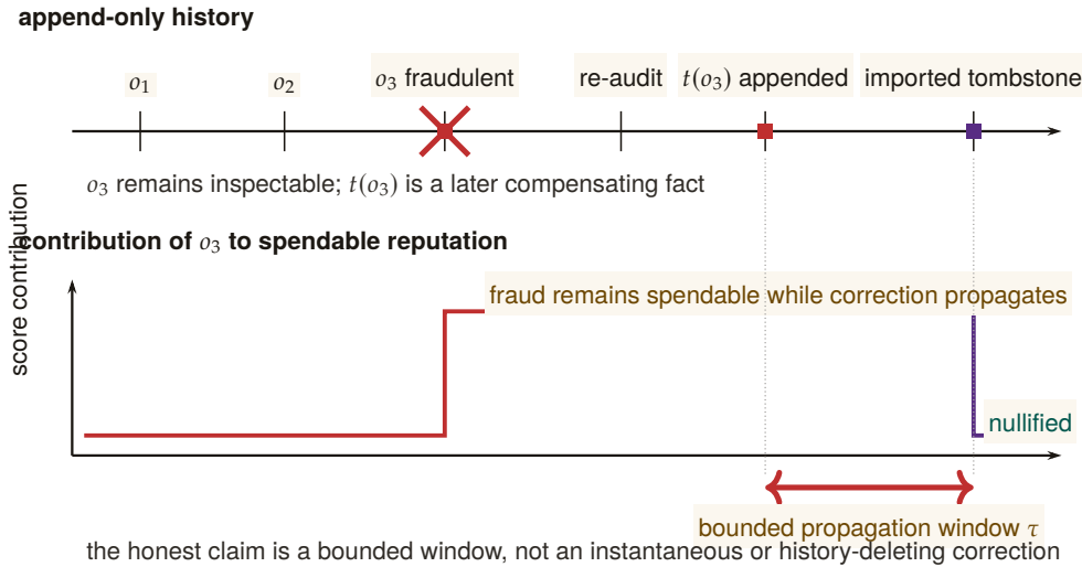
Figure 5.11. A tombstone changes score consumption without rewriting history. The upper rail remains append-only: fraudulent outcome o_3 , the overturning re-audit, and tombstone t(o_3) are all preserved as distinct facts. The lower trace shows what does change. The fraudulent contribution remains spendable until the tombstone reaches an importing harbor, then falls to zero. The measured interval \tau is the federation’s revocation-convergence obligation; the protocol bounds that interval rather than pretending it never existed.
