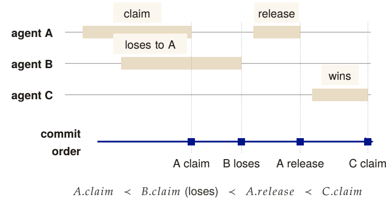
Figure 1.12. A real-time history and its extracted linearization. Operations overlap in caller time, but each receives one commit point on the single writer’s rail, and the linearization reads: A claims, B loses, A releases, C claims. The claim is conditional on one writer, no uncommitted reads, and replies after commit. [internal]
