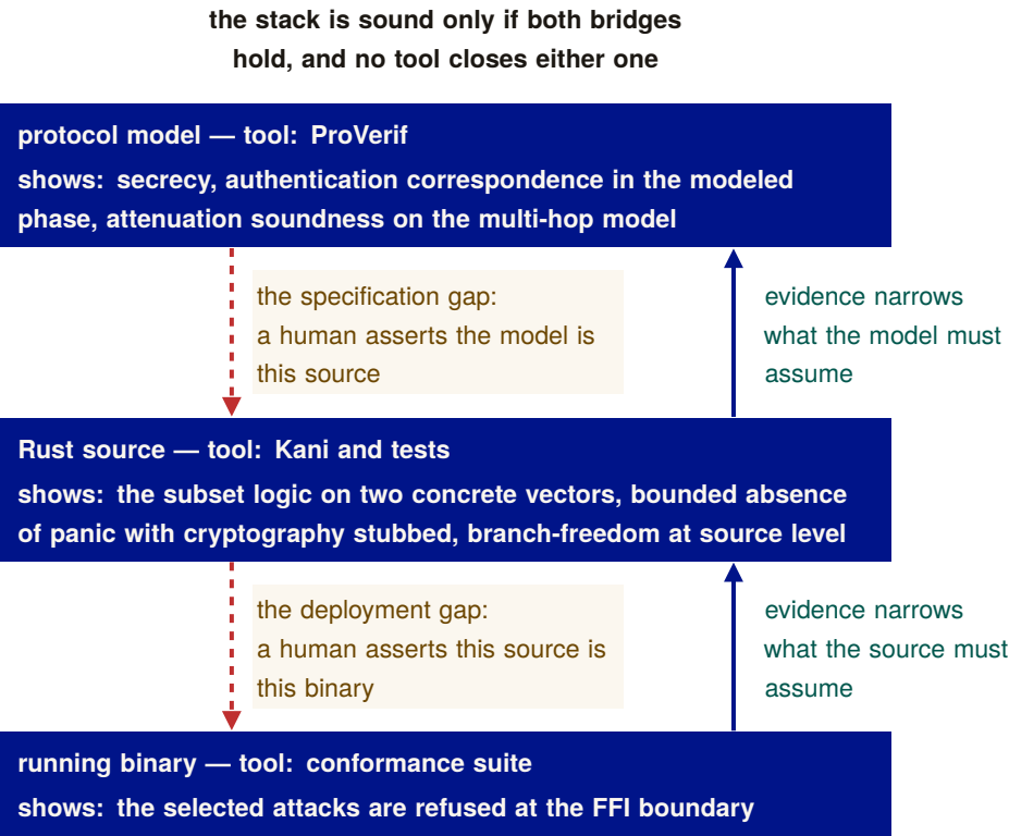
Figure 2.7. The assurance case of Table 2.2 as a chain. Obligations descend: each layer hands the next a claim it cannot discharge itself. Evidence ascends: each tool’s output narrows what the layer above must assume. The two amber gaps are the only places in the whole case where a human, not a tool, asserts that one layer’s claim carries over to the next — that the modeled protocol is this source, and that the inspected source is this running binary. [internal]
