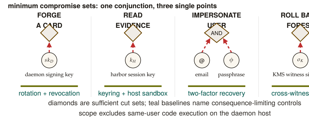
Figure 7.8. The custody theorem has four small attack cut sets rather than one undifferentiated trust boundary. Card forgery, evidence decryption, and forest rollback each have one sufficient secret; user impersonation is the sole conjunctive failure and requires both email and passphrase. The teal baselines name the consequence-limiting control for each cut. Same-user code execution remains outside the theorem because that adversary can read every secret available to the user process.
