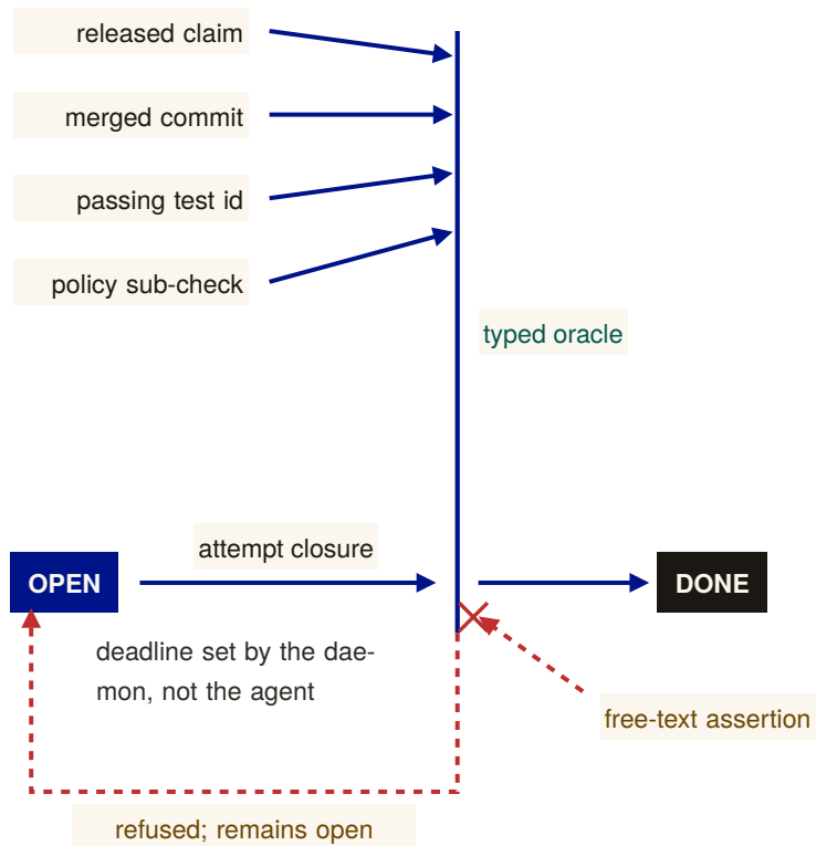
Figure 1.9: Typed evidence passes through a narrow closure aperture. A commitment closes as done only when the daemon can re-run a check from the finite oracle vocabulary: a released claim, merged commit, passing test id, or satisfied policy sub-check. A free-text assertion is refused and the commitment remains open. The deadline is set by the daemon, not the agent. [internal]
