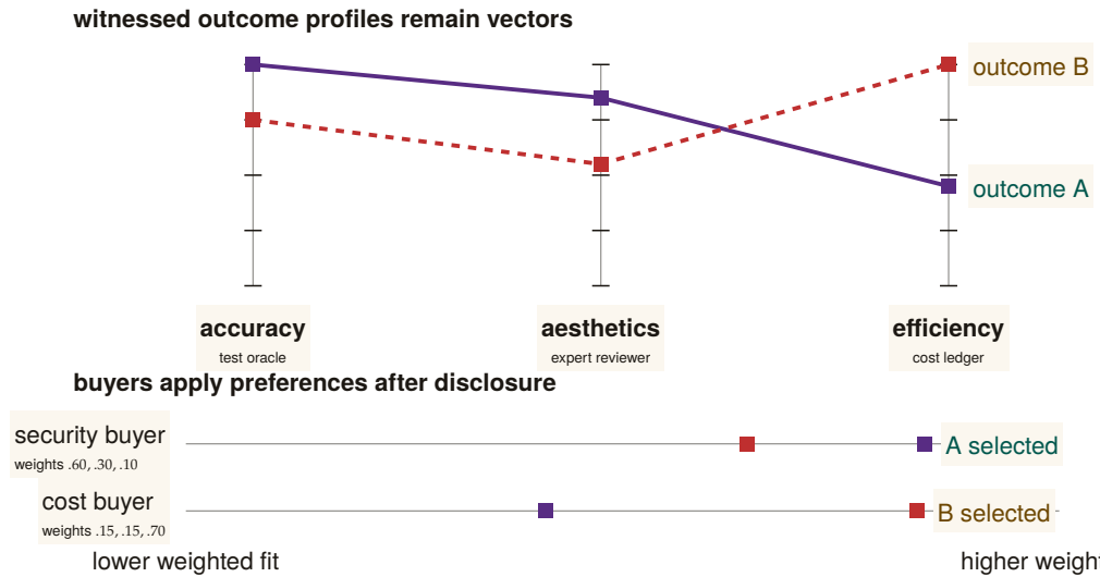
Figure 5.7. One quality vector supports legitimate preference reversal. Outcome A is strongest on accuracy and aesthetics; outcome B is strongest on efficiency. Each axis is independently judged, then disclosed without a universal scalar. A security-weighted buyer selects A while a cost-weighted buyer selects B. Premature averaging would erase one of these valid decisions and create a single Goodhart target. Color is redundant with solid-versus-dashed profiles and direct labels.
