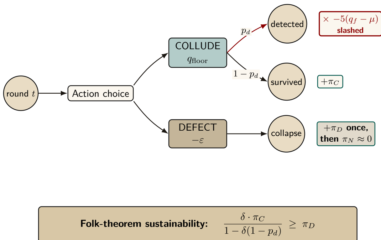
Figure 7: Cartel repeated-game node under the grim-trigger strategy. Each round a colluding member chooses between maintaining the floor q_{\text{floor}} or undercutting it by \varepsilon . Detection (probability p_d ) lands on the red \times path: the colluder is slashed -5(q_f - \mu) . One-shot defection takes the \pi_D gain once, then collapses the future \pi_C stream to \pi_N \approx 0 . The cartel is self-sustaining exactly when the inequality at the bottom holds; raising p_d (sampled adversarial re-audit) or capping \pi_C (diminishing-returns concavity on pairwise outcomes) pushes the critical discount factor past 1 and breaks it.
