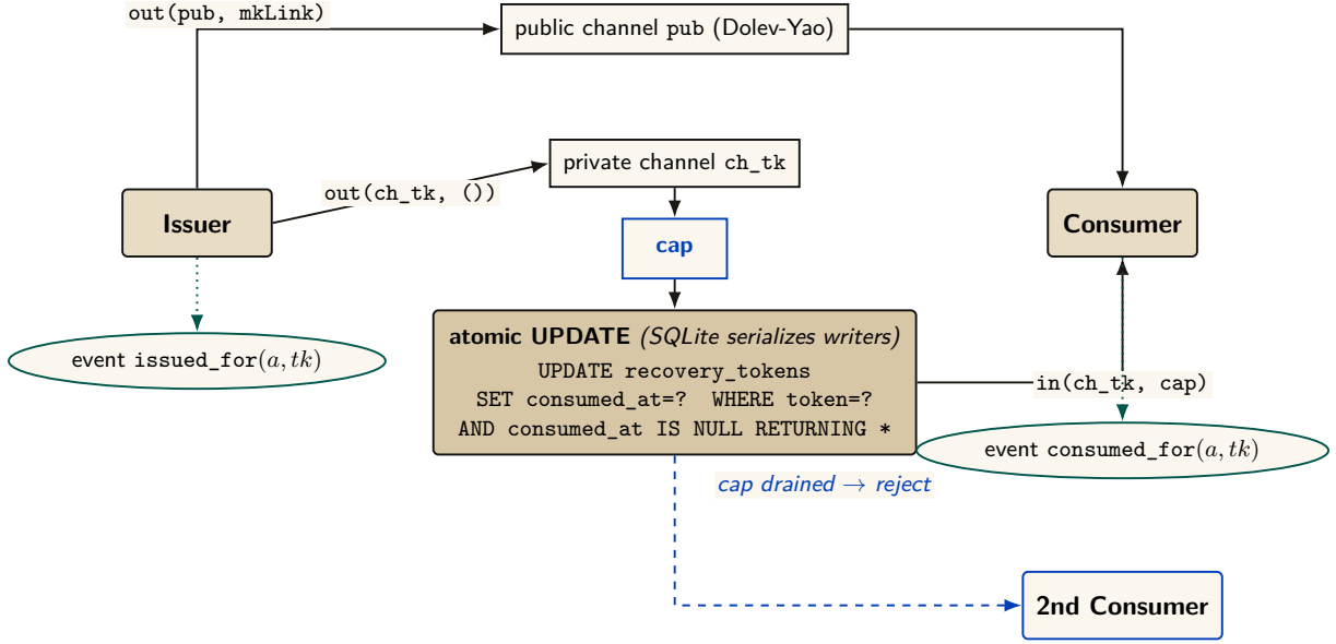
Figure 9: Magic-link single-use atomicity. The SQL UPDATE ...WHERE consumed_at IS NULL RETURNING is the runtime analogue of the ProVerif private-channel cap: SQLite serializes concurrent writers, so the first caller drains the cap and the second consumer's transaction returns zero rows. Verified properties: injective single-use ( \text{inj-event}(\text{consumed\_for}) \Rightarrow \text{inj-event}(\text{issued\_for}) ) and binding.
