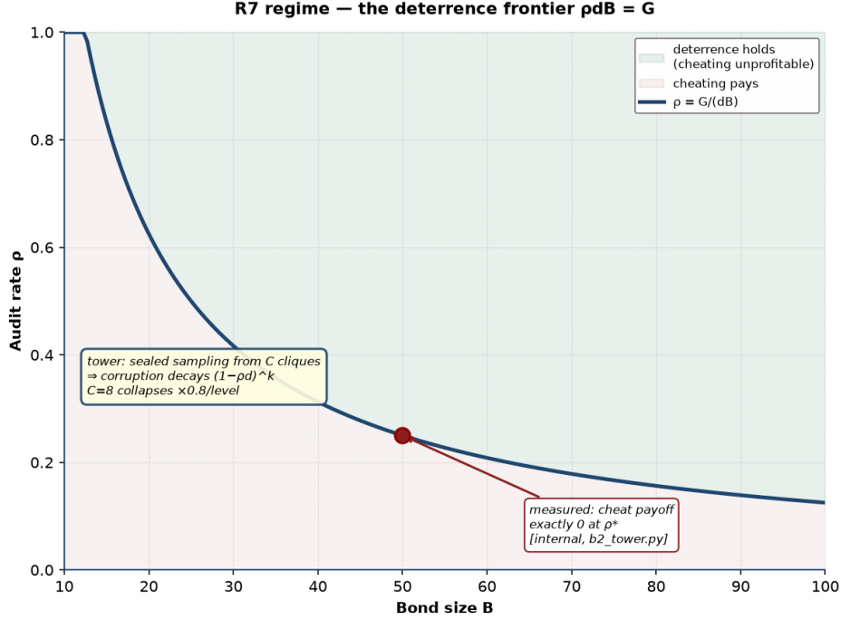
Figure 2: The regime diagram: the deterrence frontier \rho dB = G in the (bond B , audit rate \rho ) plane at G=10 , d=0.8 . Above the curve \rho = G/(dB) , cheating is unprofitable; below it, cheating pays. The marked point is the running example (B, \rho^*) = (50, 0.25) , where the measured cheat payoff is exactly zero [internal, b2.tower.py ]. The inset records the tower consequence of §4: sealed sampling from C cliques drives surviving corrupt value down as (1 - \rho d)^k , a \times 0.8 -per-level collapse at C=8 .
