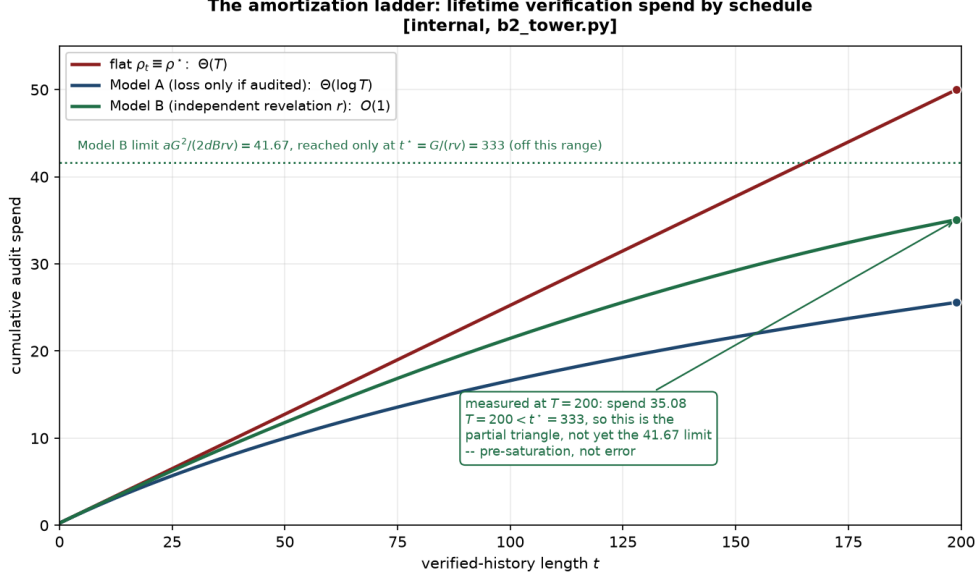
Figure 3: Cumulative audit spend against verified-history length t under the three incentive-compatible schedules of Theorem 3, at the running parameters. Flat auditing (shipped) grows linearly; Model A (harborblue) grows logarithmically; Model B (seagreen) approaches the closed-form limit aG^2/(2dBrv) = 41.67 but has not reached it by the measured horizon T=200 , since saturation requires t^* = G/(rv) = 333 — the gap between the measured 35.08 and the limit is pre-asymptotic, not error [internal, b2_tower.py].
