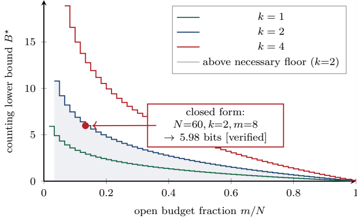
Figure 2: Regime diagram for the necessary counting floor B^* against the open-budget fraction m/N (here N=60 , k=2 ; the marked point is the experiment’s m=8 , B^*=5.98 bits [verified]). The lower bound is steep where budgets are tight and vanishes when the overseer opens everything. Points above the bound are not automatically achievable: codeword cover sets can overlap.
