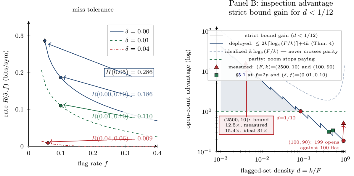
Figure 10: Panel A shows the Bernoulli rate–distortion frontier with separate miss and flag budgets, including its zero-rate region. Panel B plots the guaranteed advantage 1/[d(2\lceil\log_2(1/d)\rceil + 4)] of the specified halving procedure, with the idealized 1/[d\log_2(1/d)] for comparison. The displayed bound guarantees a strict saving for d < 1/12 and breaks even at d = 1/12 . At dense placement (F, k) = (100, 90) the measured procedure uses 199 opens against 100 flat; a bound below parity alone would not prove that loss.
