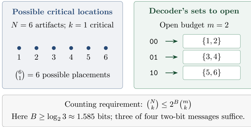
Figure 1: A complete covering in the N = 6, k = 1, m = 2 case. The three displayed messages name disjoint sets and cover every placement. The counting inequality is necessary for every codebook; overlap between sets can prevent a codebook from attaining it in other cases.
