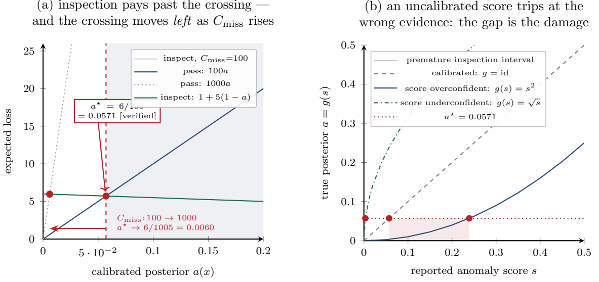
Figure 6: Regime diagram for the surfacing rule. Panel (a): expected loss of pass against expected loss of inspect, as a function of the calibrated posterior a(x) . Inspection pays exactly where the two loss lines cross, at a^* = (c_{\text{att}} + C_{\text{fa}})/(C_{\text{miss}} + C_{\text{fa}}) — the closed form obtained by solving Theorem 3’s inequality directly. At the shown costs ( C_{\text{miss}}=100 , c_{\text{att}}=1 , C_{\text{fa}}=5 ) that is 6/105 \approx 0.057 ; raising C_{\text{miss}} to 1000 moves the crossing left , to 6/1005 \approx 0.006 [verified] — the counterintuitive direction, drawn rather than asserted. Panel (b): threshold the reported score s only after calibrating the true posterior g(s) . When g(s) = s^2 , the naive rule s \geq 0.057 inspects too early: the true posterior is only about 0.00327 there; the correct score threshold is s \geq \sqrt{0.05714} \approx 0.239 . The shaded interval [0.057, 0.239] is unnecessary inspection. For g(s) = \sqrt{s} , the correct score threshold is about 0.00327 and the naive rule acts too late.
