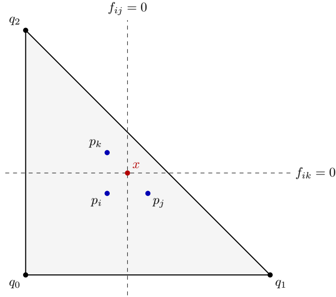
Figure 2: An F vertex: where the plane of the triangle meets two bisectors at once. Drawn in the triangle's plane, with the numbers of the worked example (§6.3).
