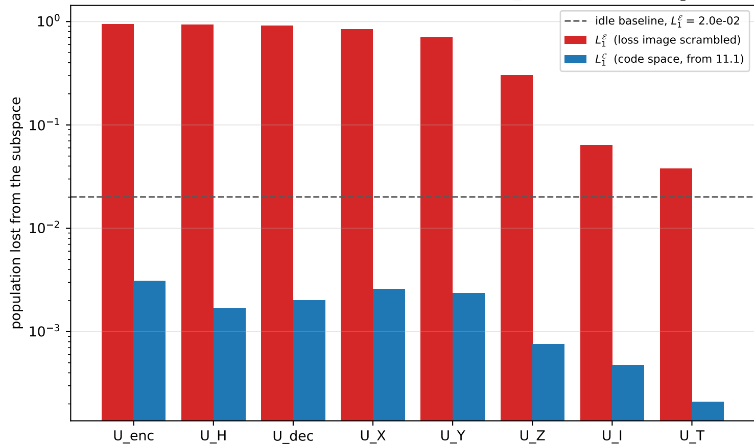
Code space vs. single-photon-loss subspace ( n_c=24 , ordered by L_1^\mathcal{E} )
