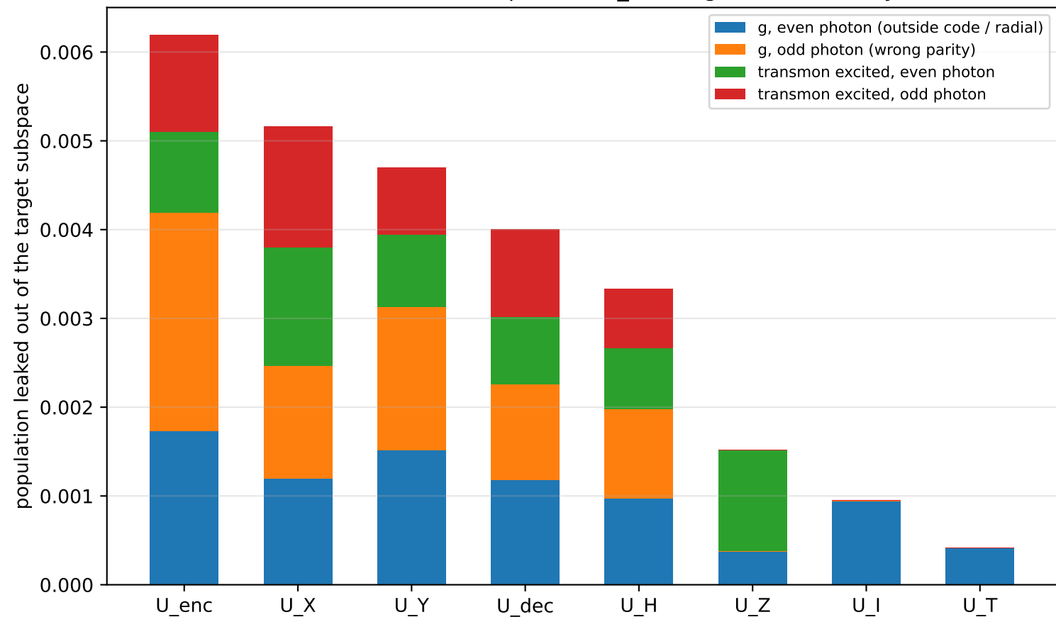
Destination of leaked amplitude ( n_c=24 , gates ordered by L1)
