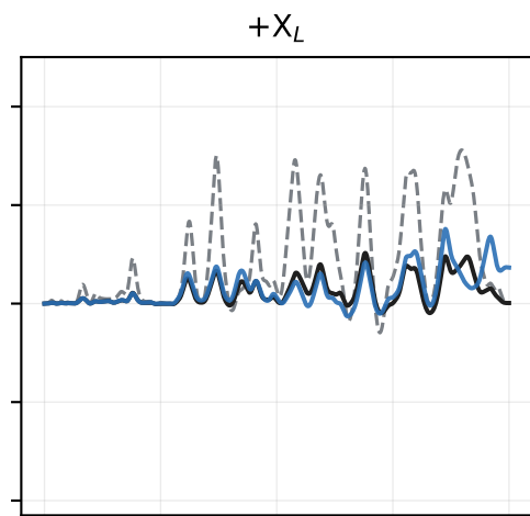
X gate: mean photon number of the code and error subspaces under U(t)
