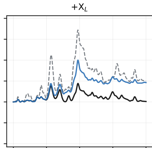
H gate: mean photon number of the code and error subspaces under U(t)
