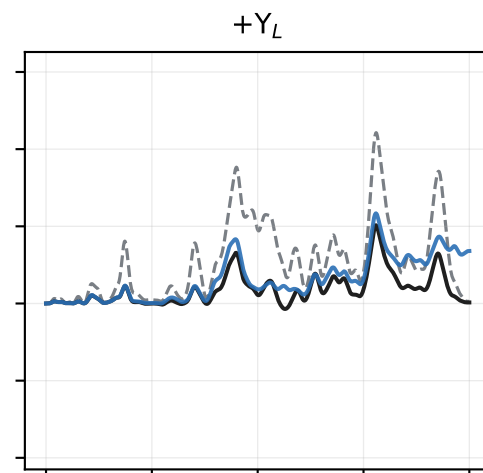
X gate: mean photon number of the code and error subspaces under U(t)
