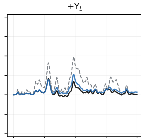
H gate: mean photon number of the code and error subspaces under U(t)
