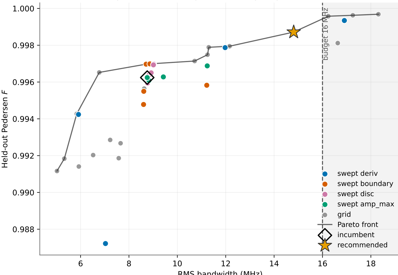
Penalty Pareto front: reported fidelity vs pulse bandwidth
