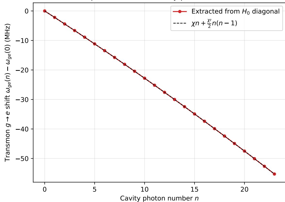
Dispersive shift vs. cavity photon number
