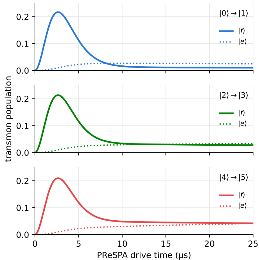
(c) Transmon excitation during correction
