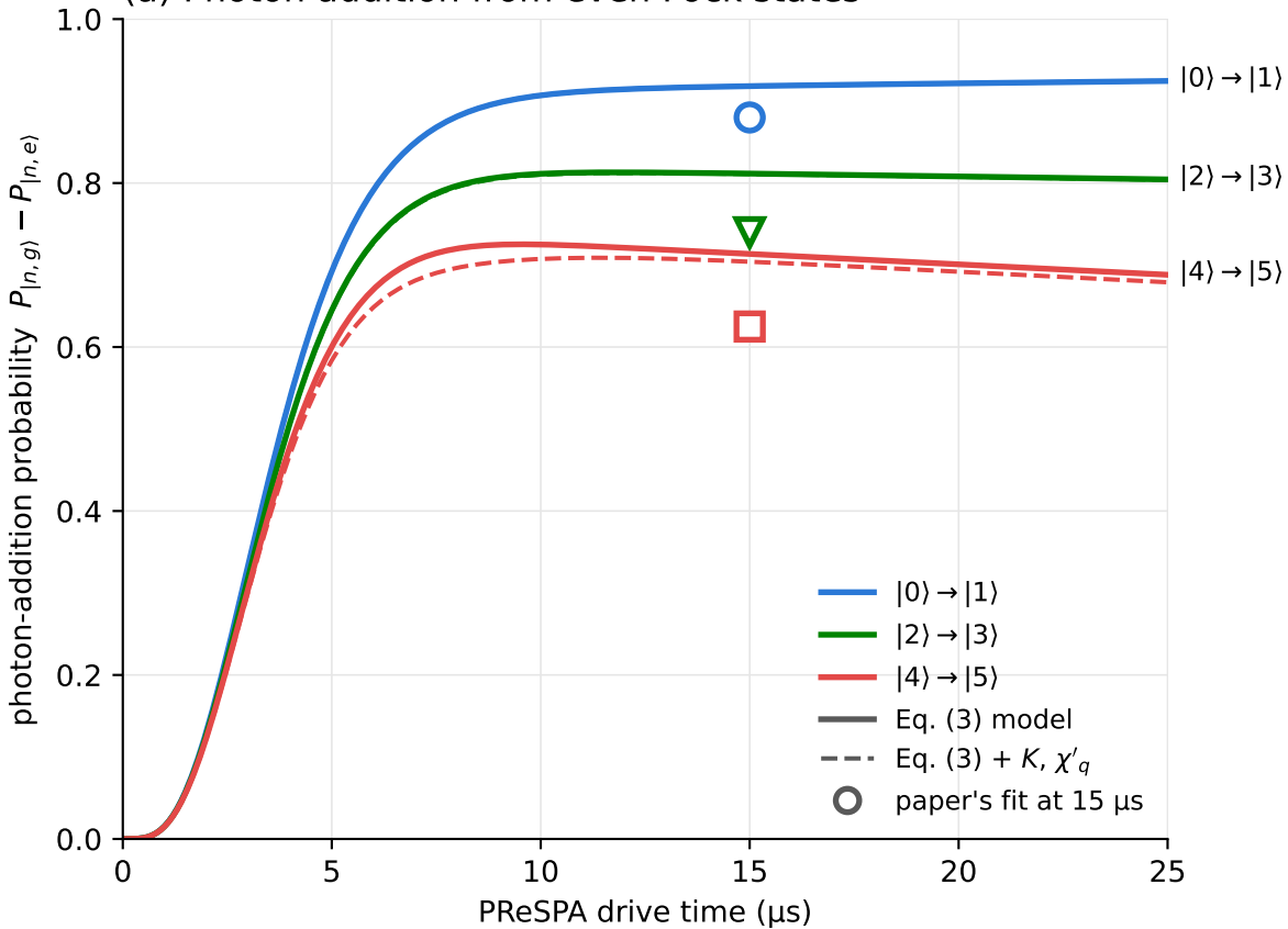
(a) Photon addition from even Fock states
