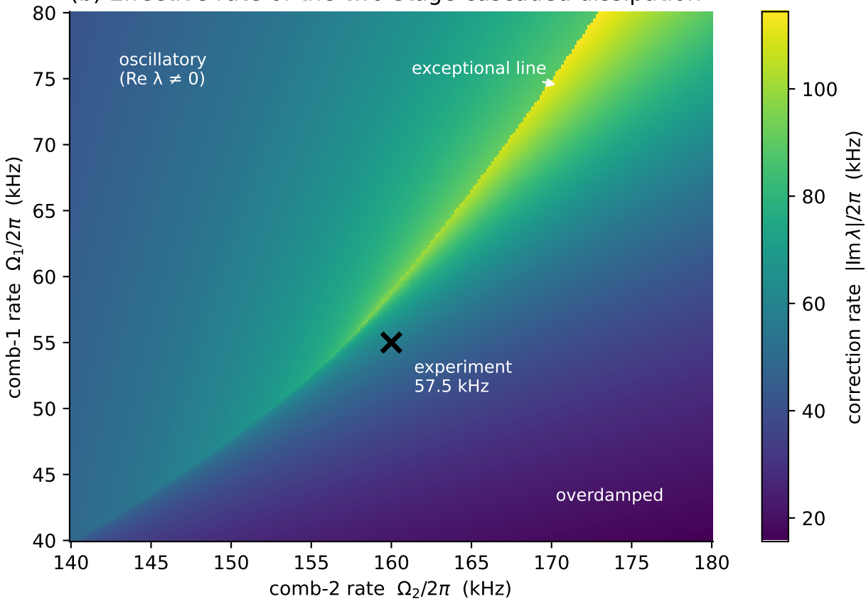
(b) Effective rate of the two-stage cascaded dissipation
