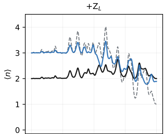
X gate: mean photon number of the code and error subspaces under U(t)
