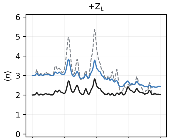
H gate: mean photon number of the code and error subspaces under U(t)
