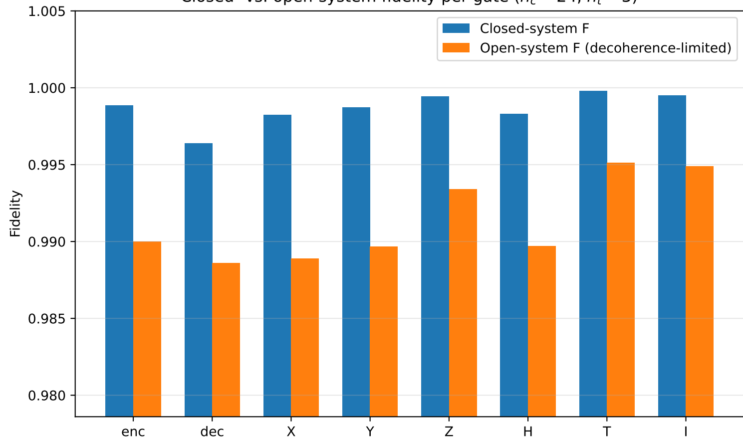
Closed- vs. open-system fidelity per gate ( n_c = 24 , n_t = 3 )
