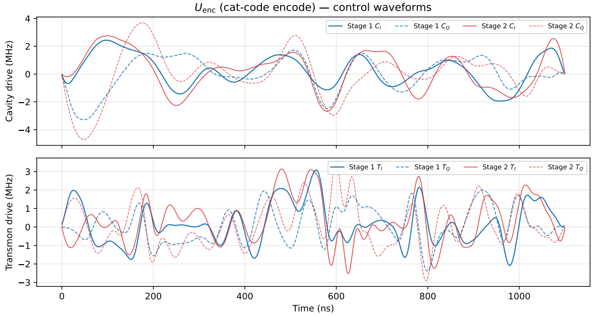
Figure 5: Control waveforms for U_{\text{enc}} : Stage 1 ( dt = 2 \text{ ns} ) vs Stage 2 ( dt = 0.2 \text{ ns} ). Solid: I channels; dashed: Q .
