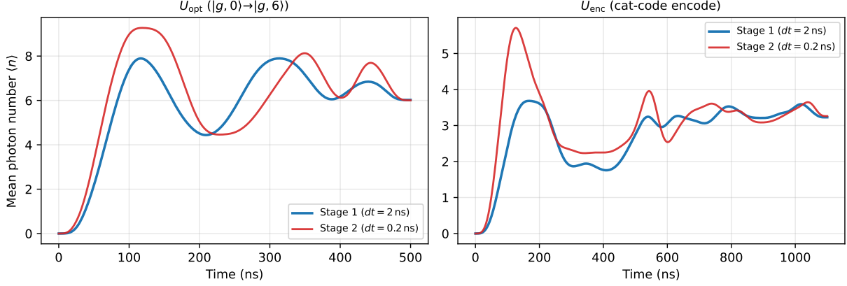
Figure 2: Mean photon number \langle n \rangle(t) at n_c = 24 . Left: U_{\text{opt}} (both stages end near \langle n \rangle = 6 ). Right: U_{\text{enc}} , |g, 0\rangle branch.
