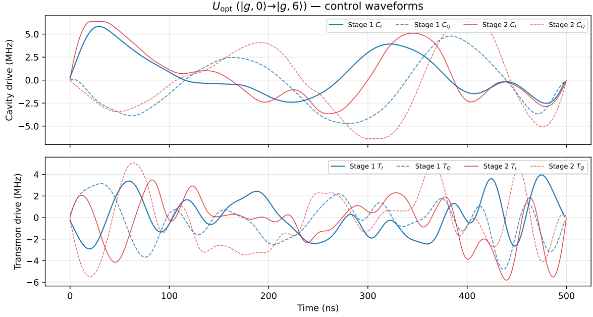
Figure 4: Control waveforms for U_{\text{opt}} : Stage 1 ( dt = 2 \text{ ns} ) vs Stage 2 ( dt = 0.2 \text{ ns} ). Solid: I channels; dashed: Q .
