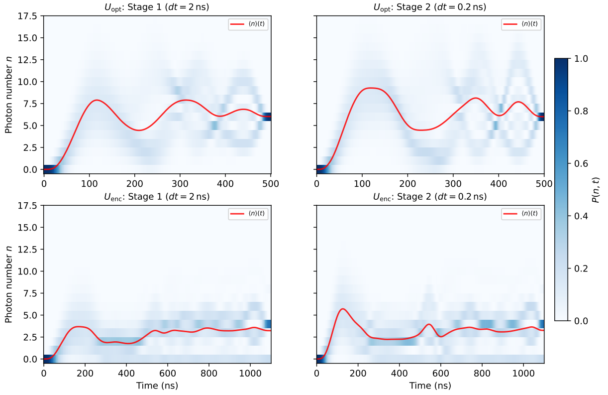
Figure 3: Fock population P(n, t) at n_c = 24 . Top row: U_{\text{opt}} ; bottom row: U_{\text{enc}} ( |g, 0\rangle branch). Left column: Stage 1; right column: Stage 2. Red curve: \langle n \rangle(t) .
