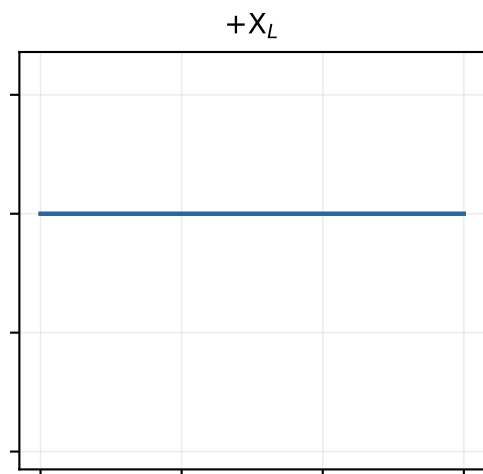
T gate: mean photon number of the code and error subspaces under U(t)
