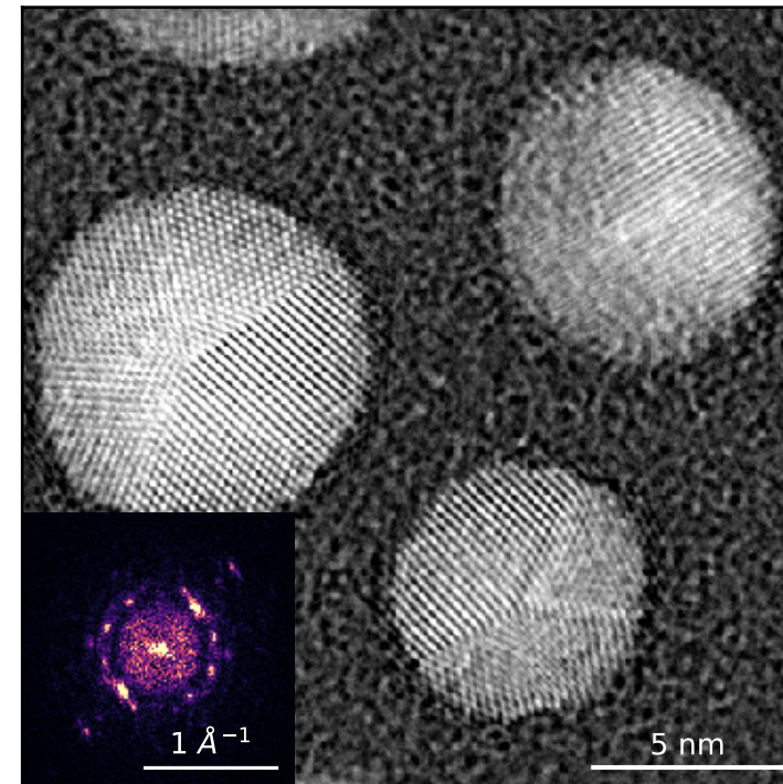
parallax imaging
