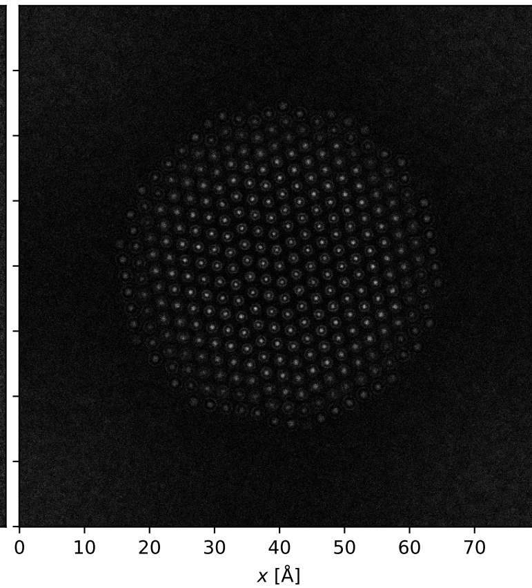
d) Zernike phase contrast
