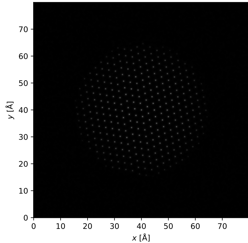
a) projected potential (ground truth)
