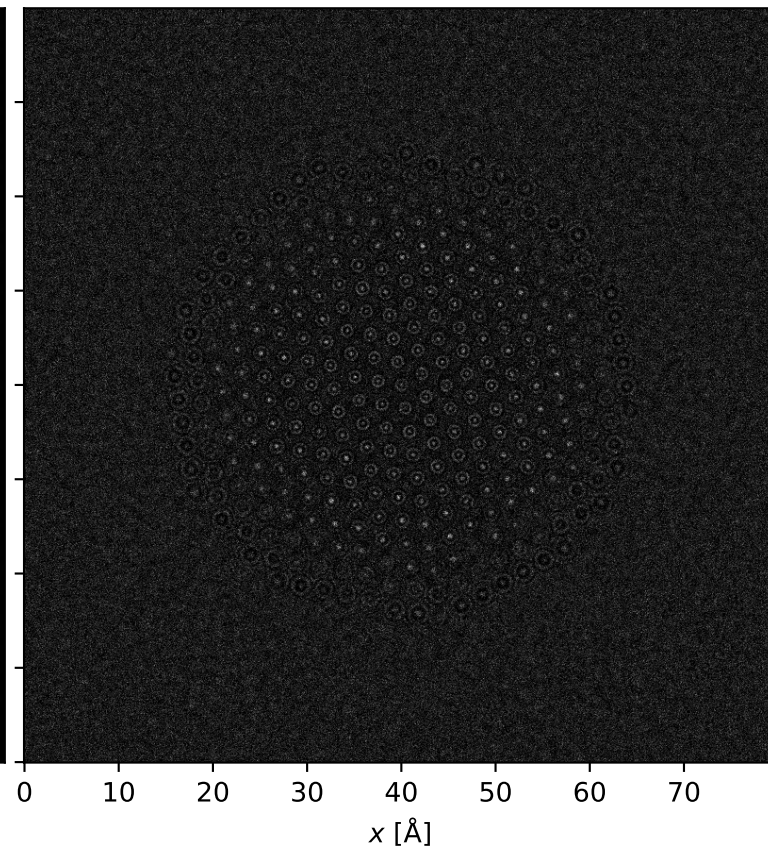
a) projected potential (ground truth)
