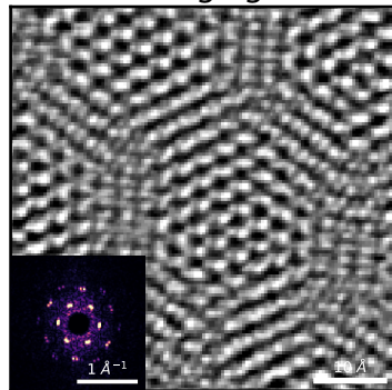
integrated center-of-mass imaging
