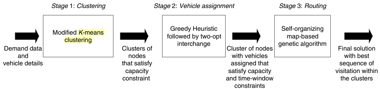
Figure 2: This schematic model of the solution highlights the structure, input, and output of the three-stage decomposition heuristic that is executed for each k value (i.e., number of vehicles).
