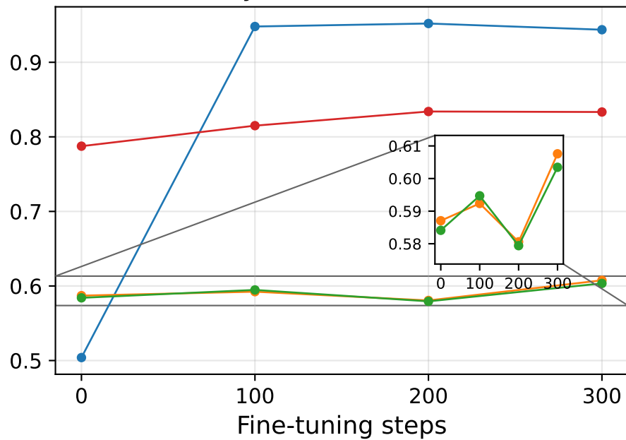
Synthetic dataset
