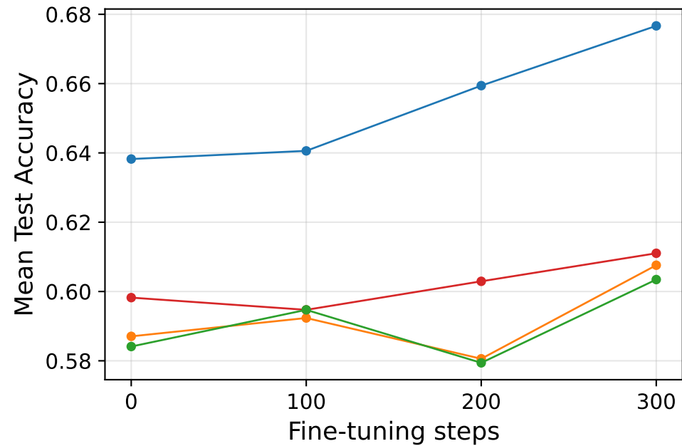
Real dataset
