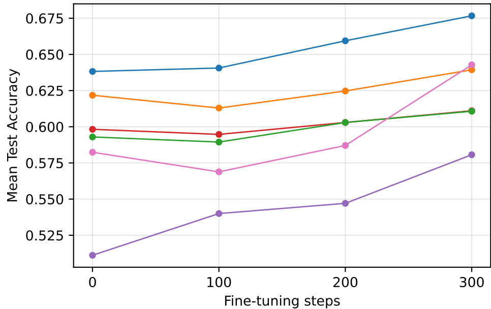
Real dataset
