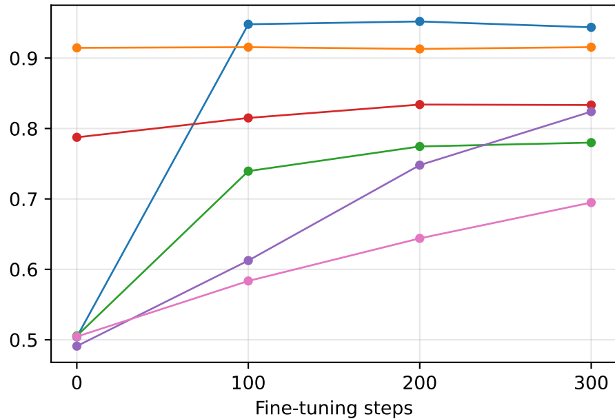
Synthetic dataset
