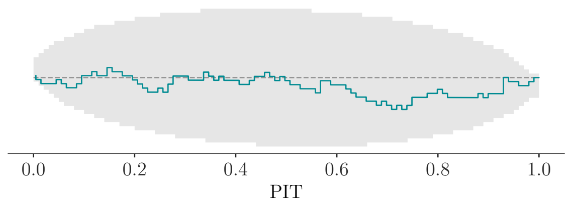
log_Ne_a (approximate)
